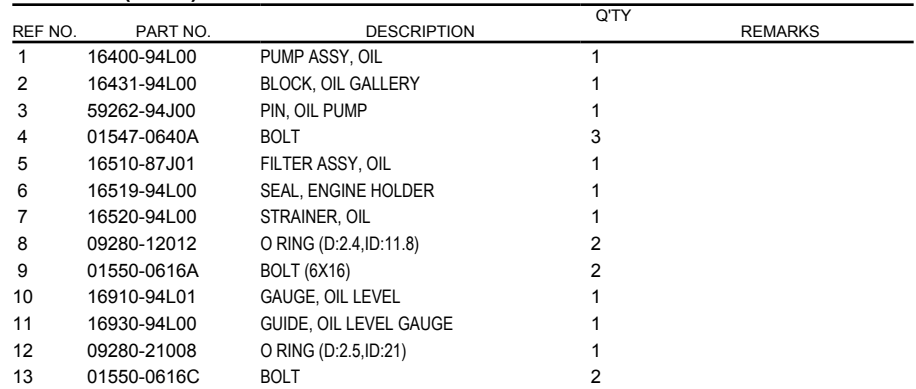
FIG.175A (1-D-6) OIL PUMP
