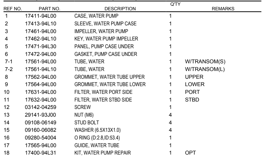
FIG.160B (1-C-12) WATER PUMP (DF30A)
