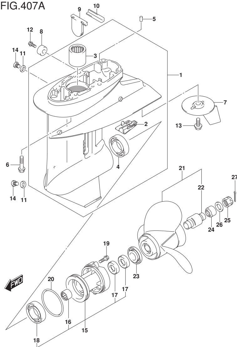
FIG.407A (1-H-13) GEAR CASE (DF25A,DF25AR,DF30AR)
