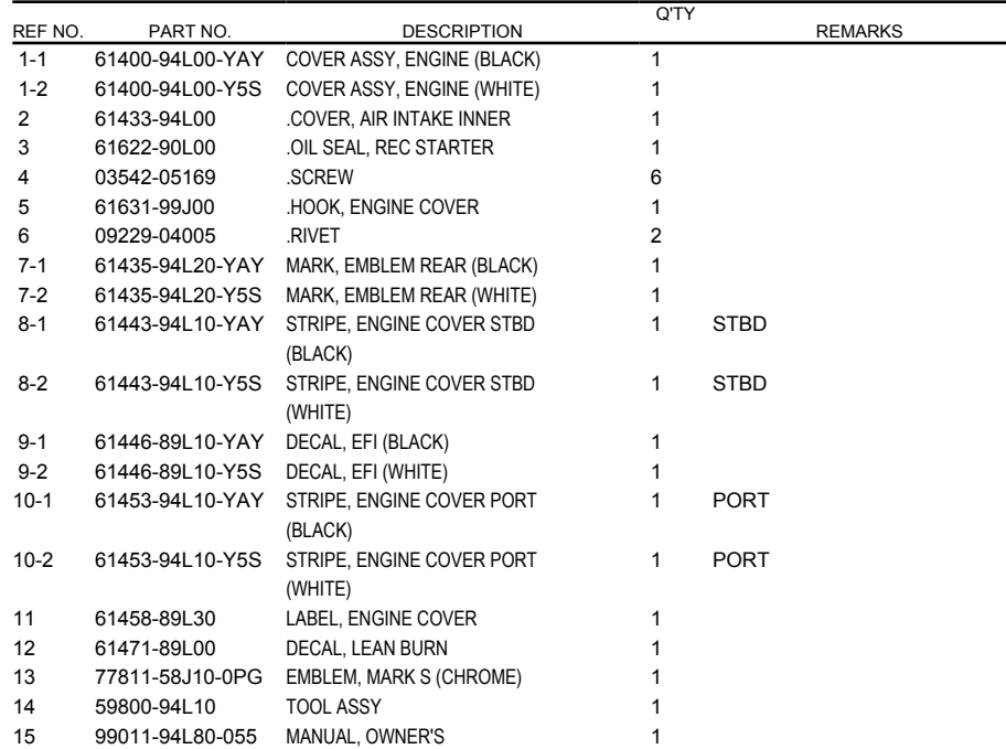
FIG.420B (1-J-2) ENGINE COVER (020:(DF25AT,DF25ATH))
