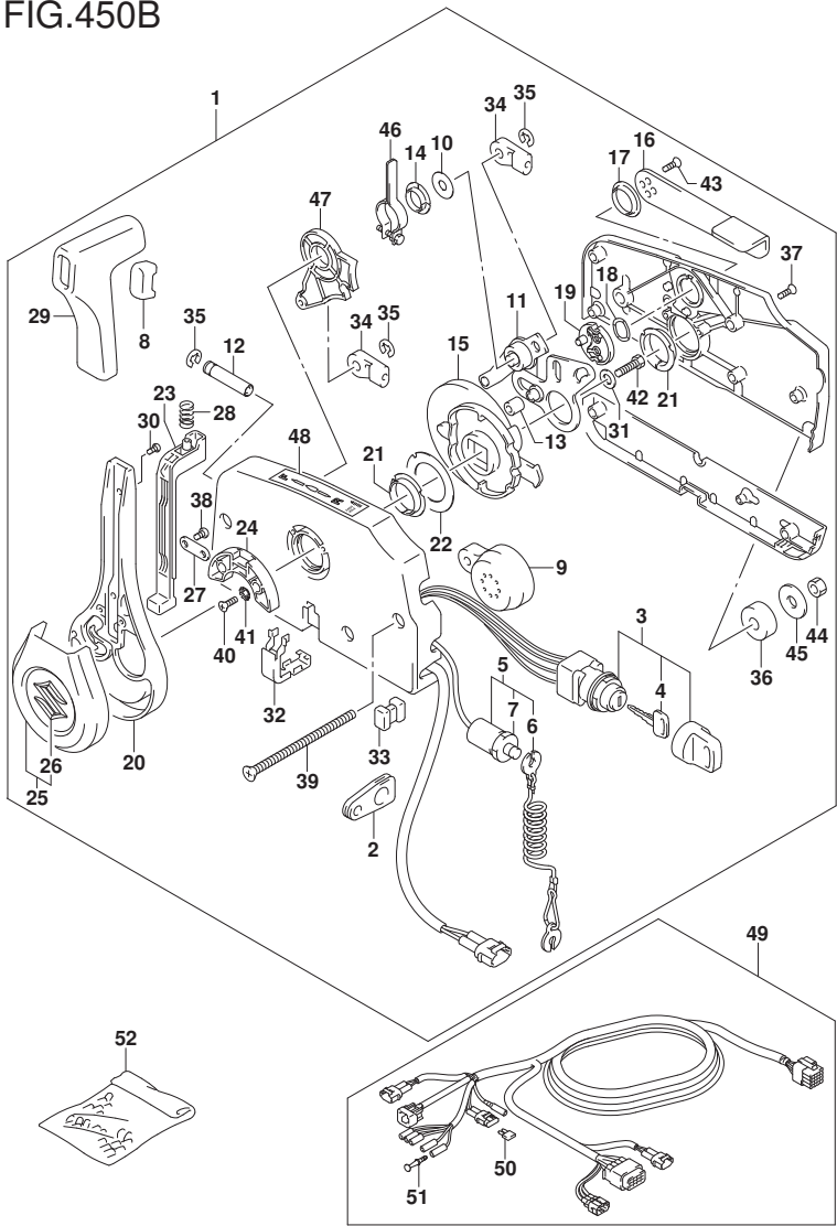
FIG.450B (1-K-4) REMOTE CONTROL (DF30AR:022)
