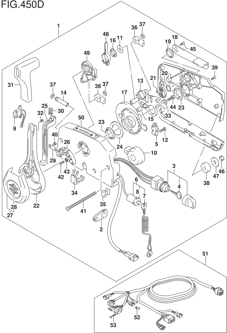
FIG.450D (1-K-9) REMOTE CONTROL ((DF25AT,DF30AT):022)
