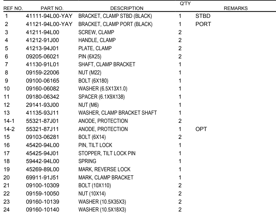
FIG.335A (1-F-14) CLAMP BRACKET (DF25A,DF25AR,DF30AR)
