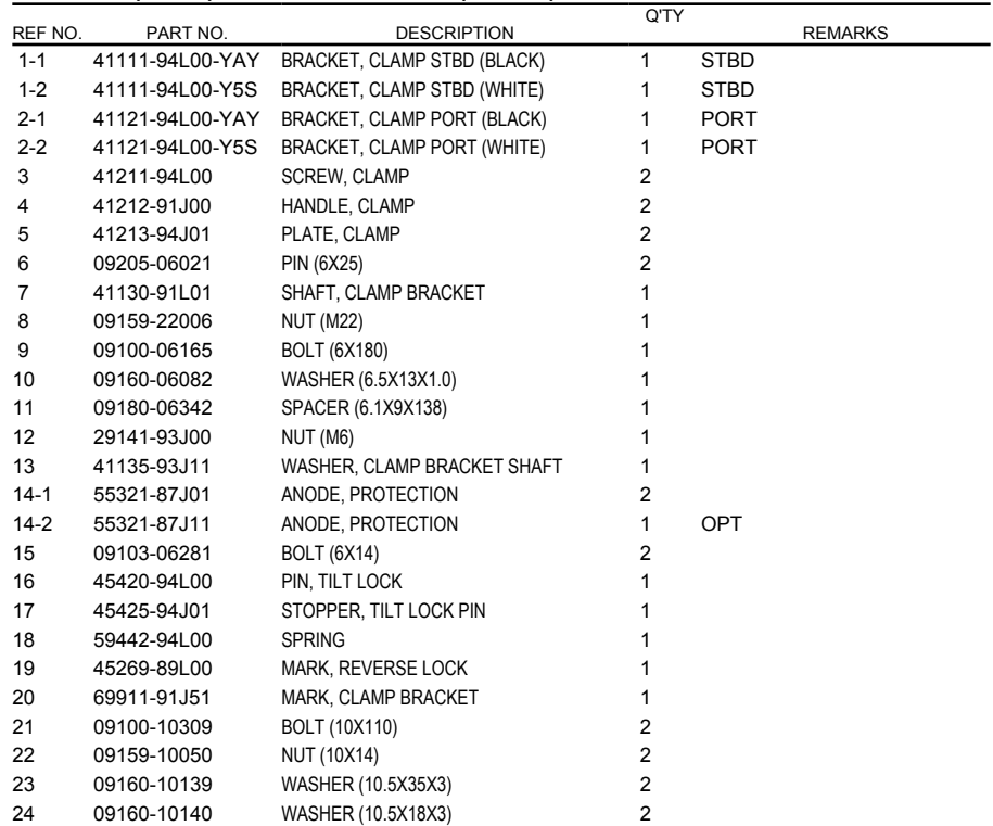
FIG.335C (1-G-3) CLAMP BRACKET (DF30A)
