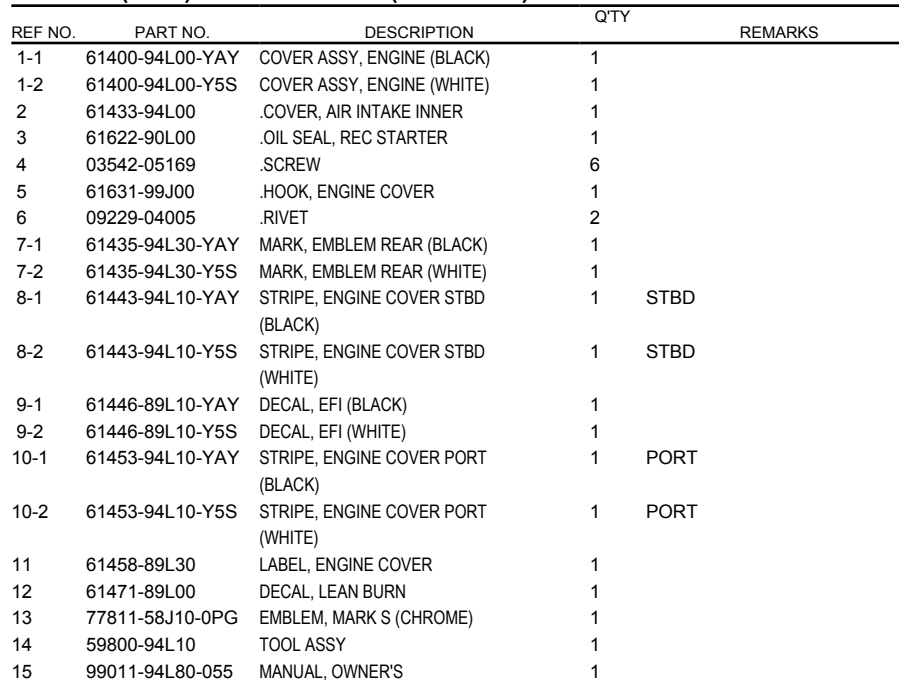
FIG.420E (1-J-5) ENGINE COVER (020:DF30A)
