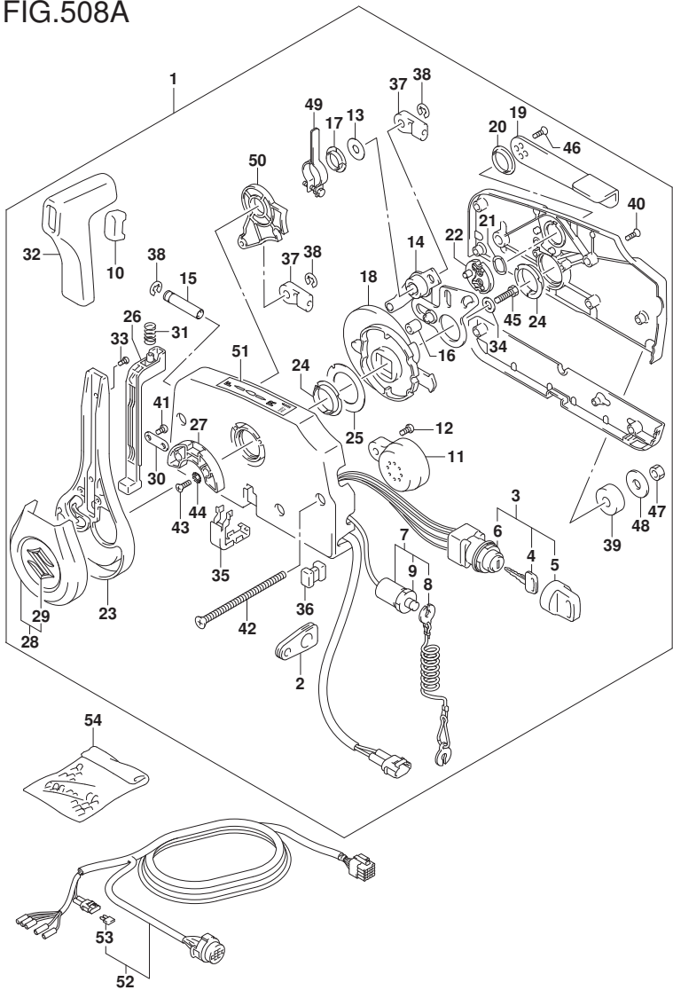
FIG.508A (1-K-15) OPT:REMOTE CONTROL (SEE NOTE)
