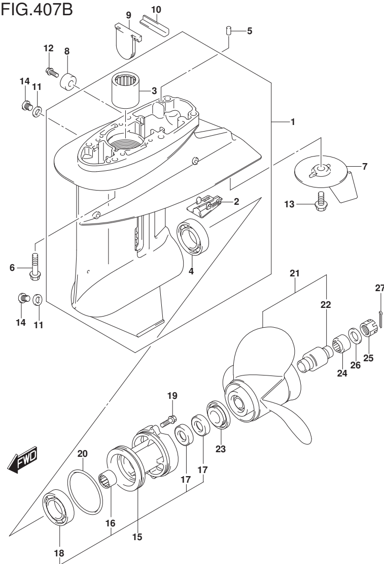
FIG.407B (1-H-14) GEAR CASE (DF25AT,DF25ATH,DF30A,DF30AT,DF30ATH)
