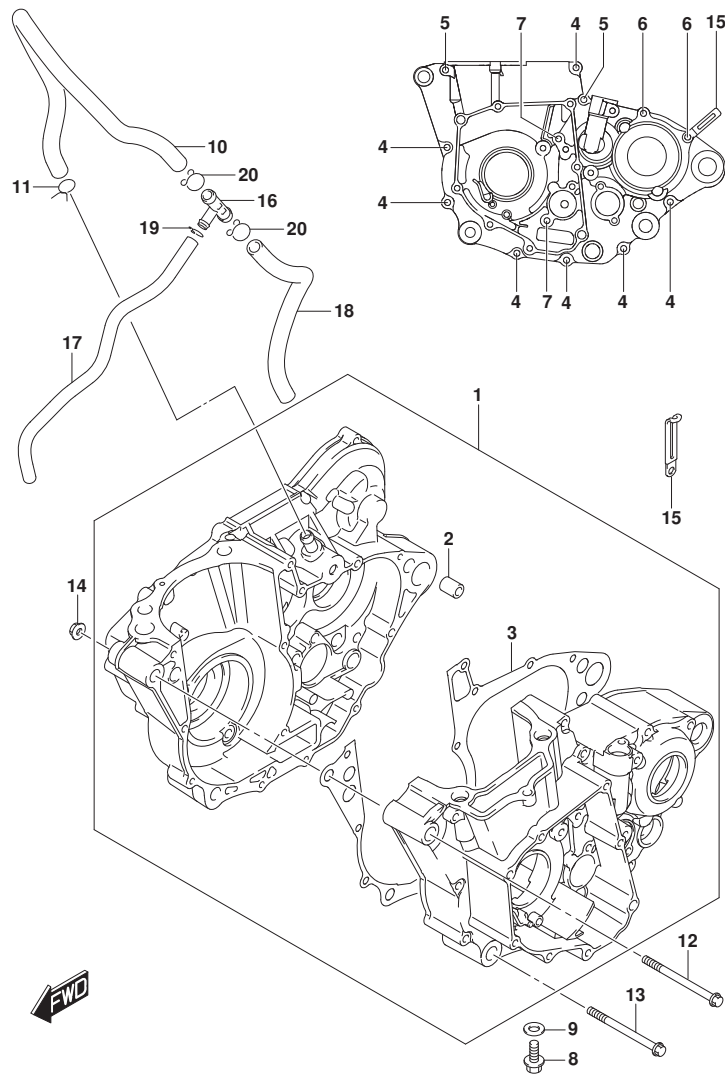
RM-Z450M0_E19_108A CRANKCASE
