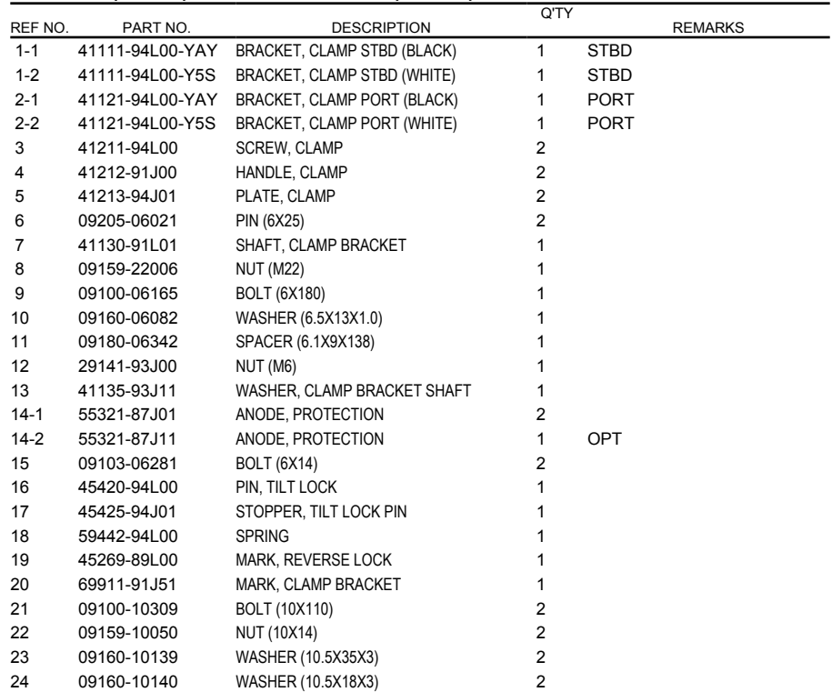
FIG.335C (1-F-11) CLAMP BRACKET (DF30A)
