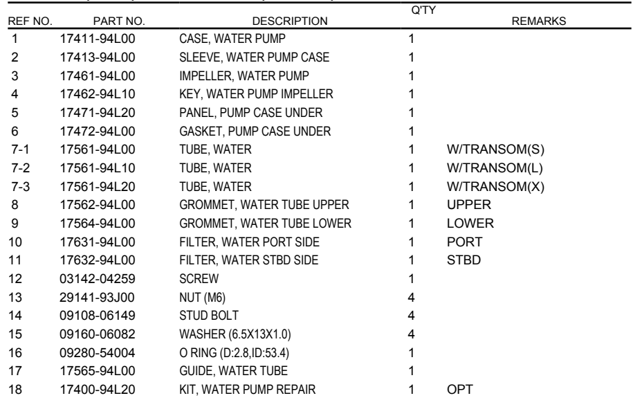
FIG.160C (1-C-8) WATER PUMP (DF30AQ)
