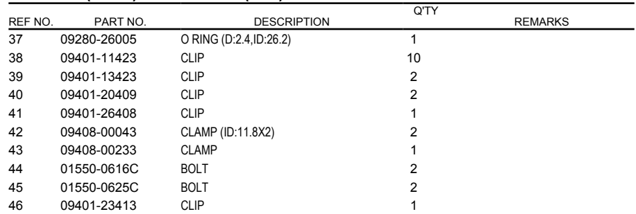
FIG.146A (1-C-3) FUEL PUMP (P01)
