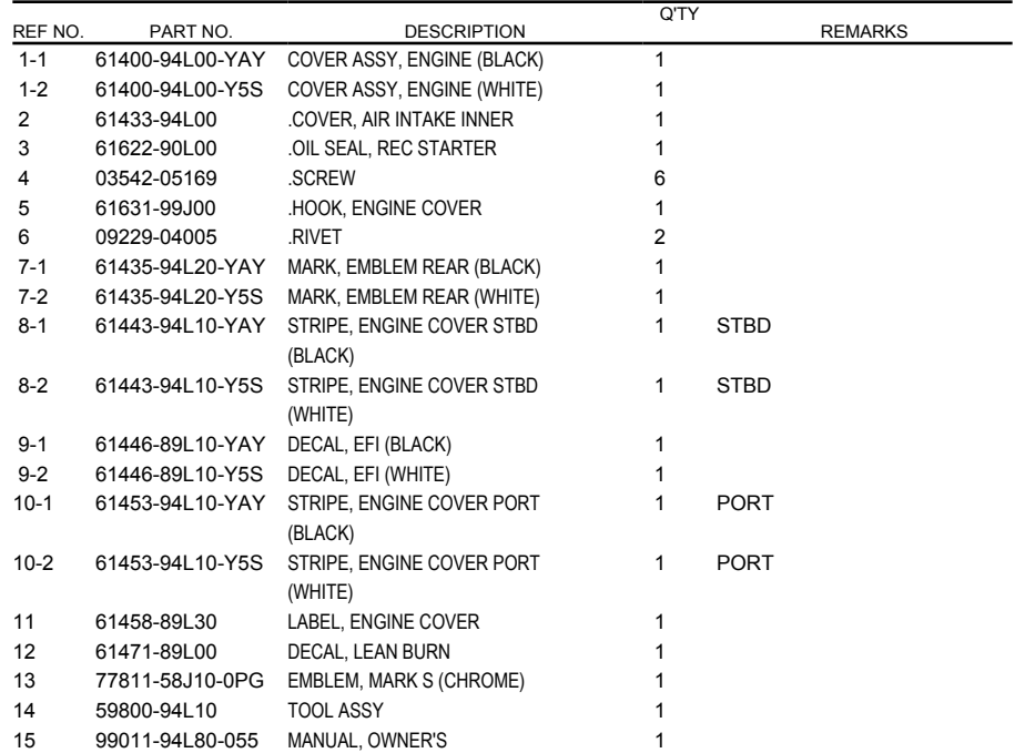
FIG.420B (1-I-11) ENGINE COVER ((DF25AT,DF25ATH):020)
