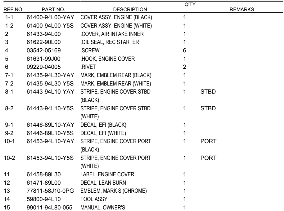
FIG.420D (1-I-13) ENGINE COVER (DF30A:020)
