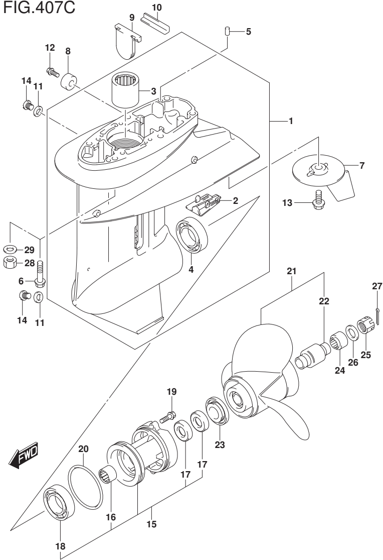
FIG.407C (1-H-12) GEAR CASE (DF30AQ)
