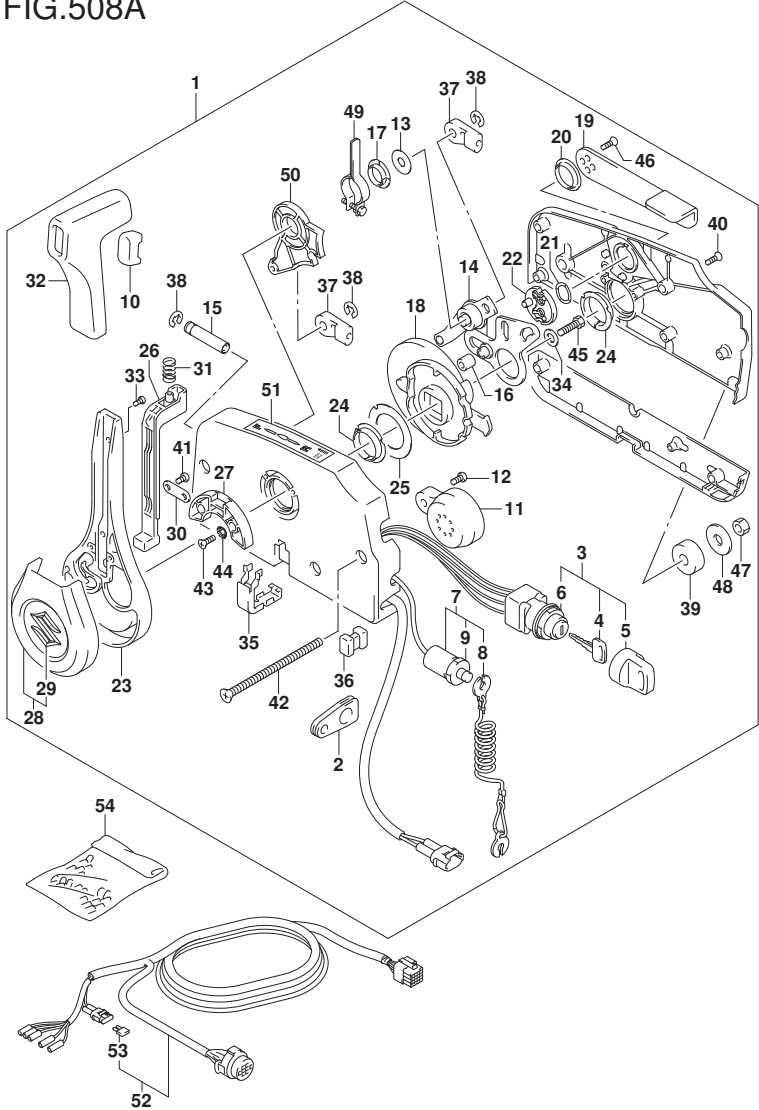
DF25A_30A_P01_021_508A OPT:REMOTE CONTROL
