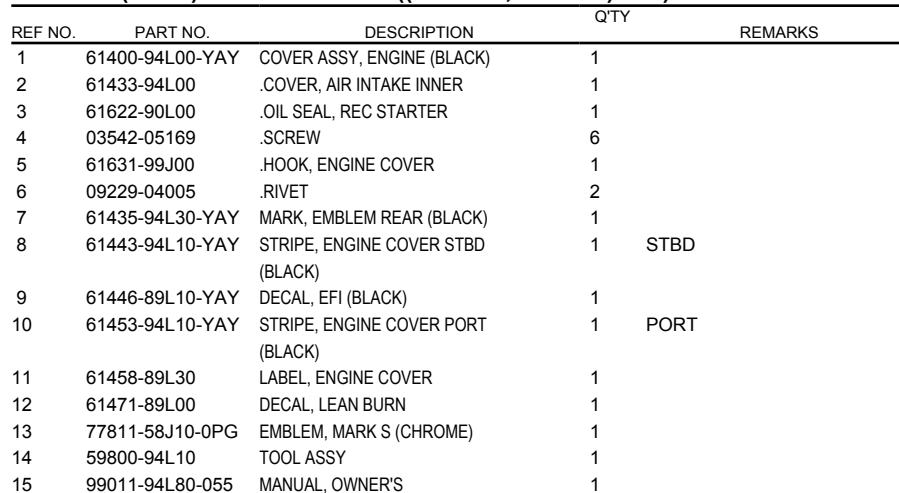
FIG.420E (1-I-14) ENGINE COVER ((DF30AR,DF30AQ):020)
