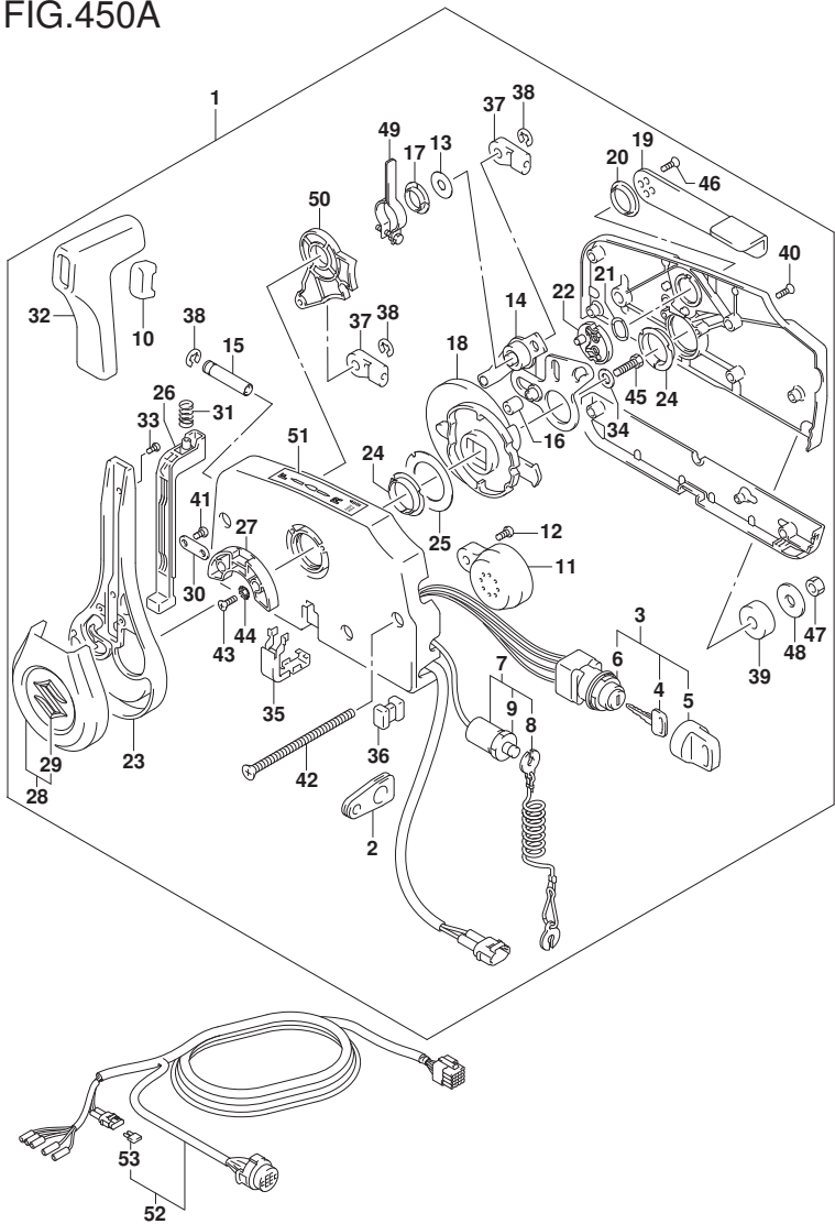
FIG.450A (1-J-11) REMOTE CONTROL (DF25AR,DF30AR)
