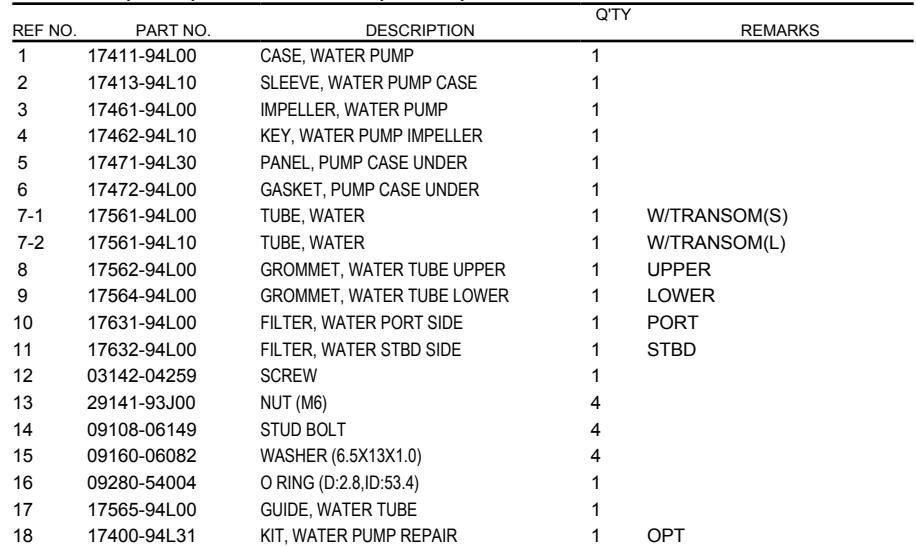
FIG.160B (1-C-7) WATER PUMP (DF30A)
