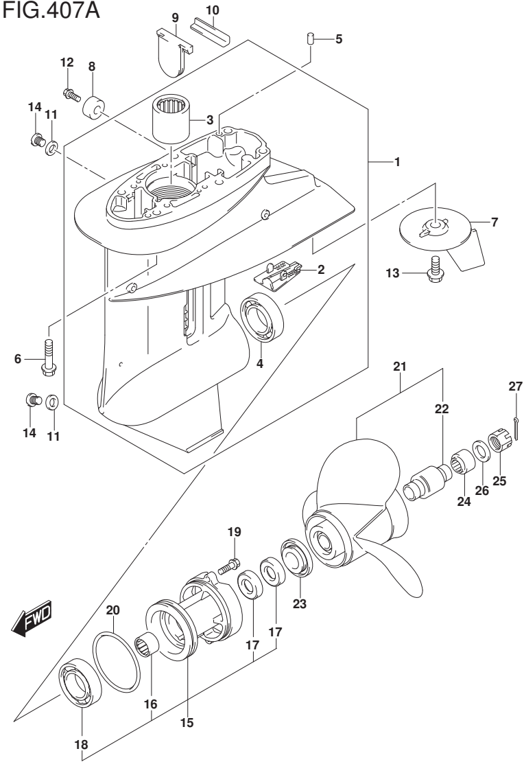
FIG.407A (1-H-7) GEAR CASE (DF25A,DF25AR,DF30AR)
