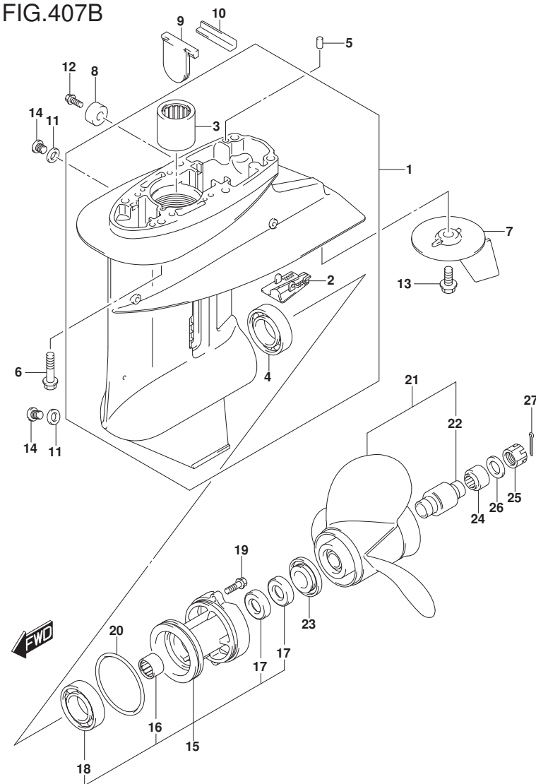
FIG.407B (1-H-9) GEAR CASE (DF25AT,DF25ATH,DF30A,DF30AT,DF30ATH)
