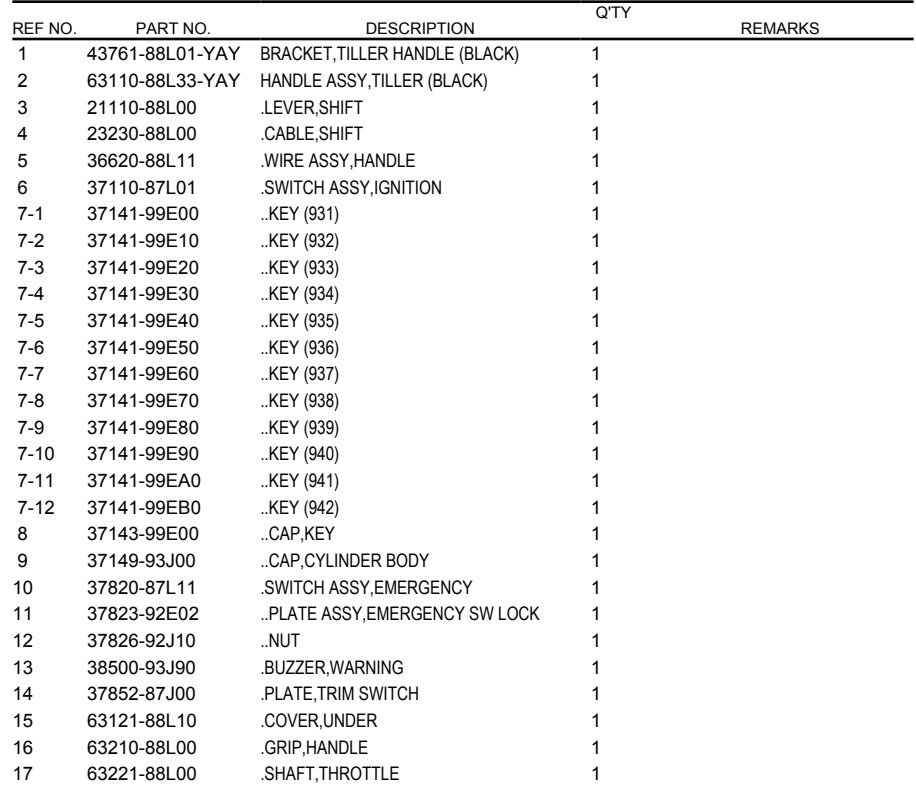
FIG.444A (1-O-12) TILLER HANDLE (DF40AQH,DF60AQH)
