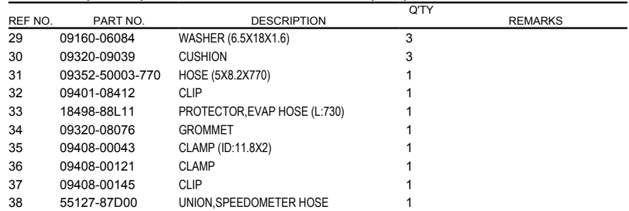
FIG.143B (1-C-11) FUEL VAPOR SEPARATOR (E40)
