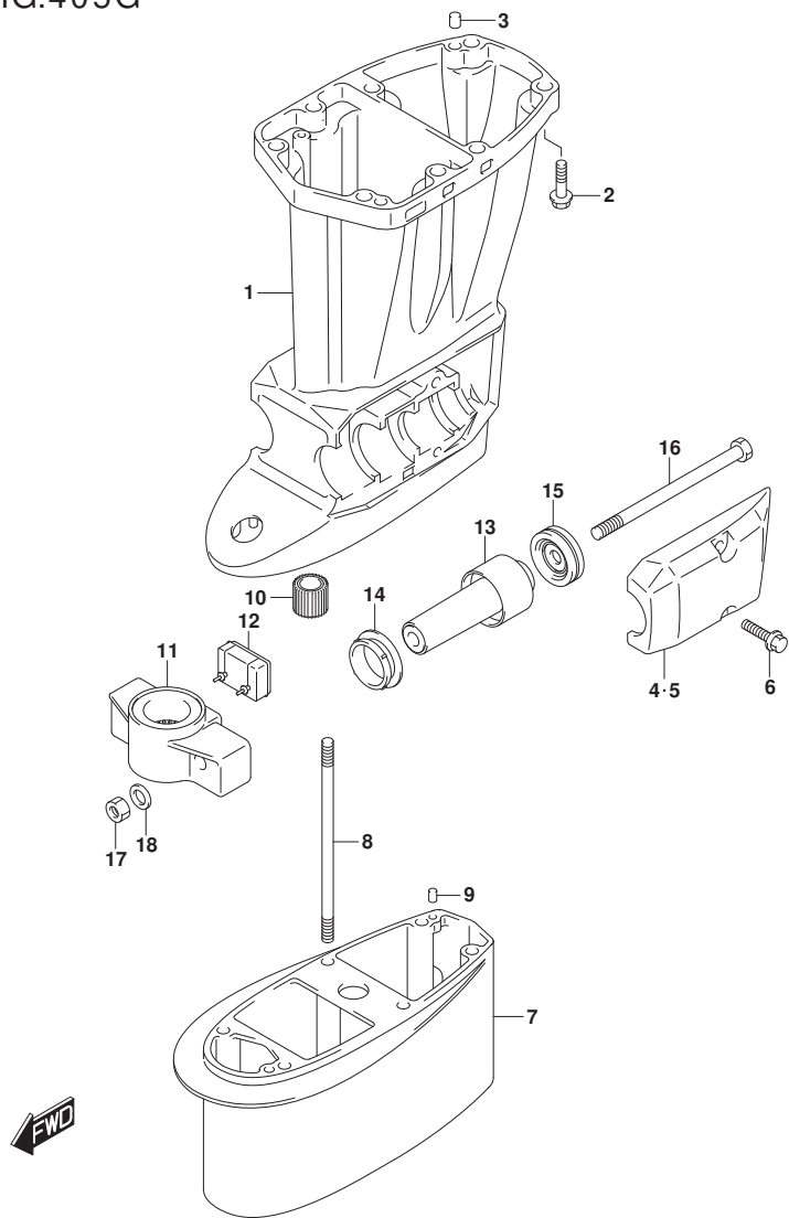
DF60A_E01_020_405G DRIVE SHAFTHOUSING
