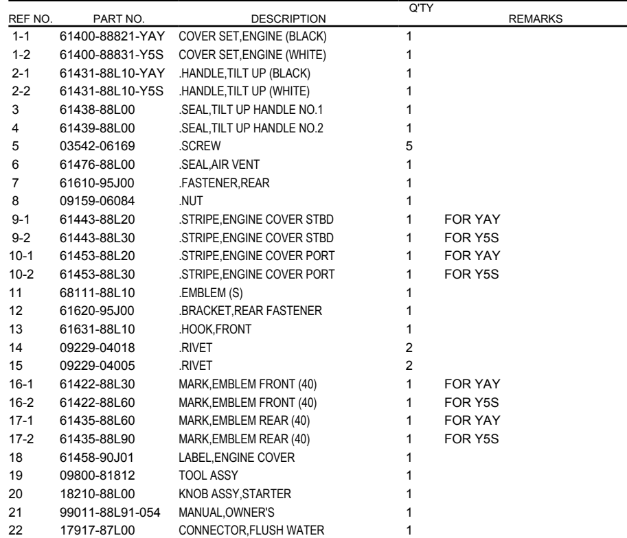
FIG.420C (1-O-3) ENGINE COVER (DF40AST:E34,DF40ASVT)
