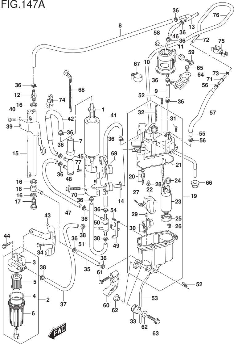
DF250_E01_020_147A FUEL PUMP/FUEL VAPOR SEPARATOR
