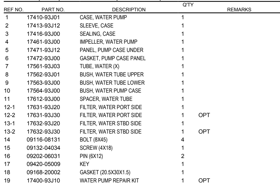
FIG.160D (1-D-7) WATER PUMP (DF200Z E40)
