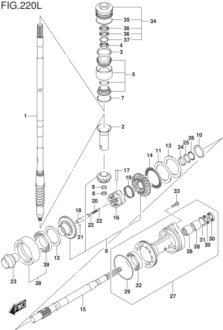
FIG.220L (1-H-10) TRANSMISSION (DF250Z E40)
