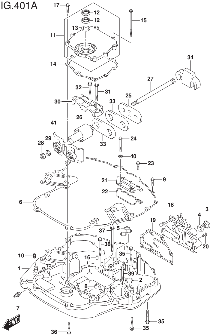
DF250_E01_020_401A ENGINE HOLDER
