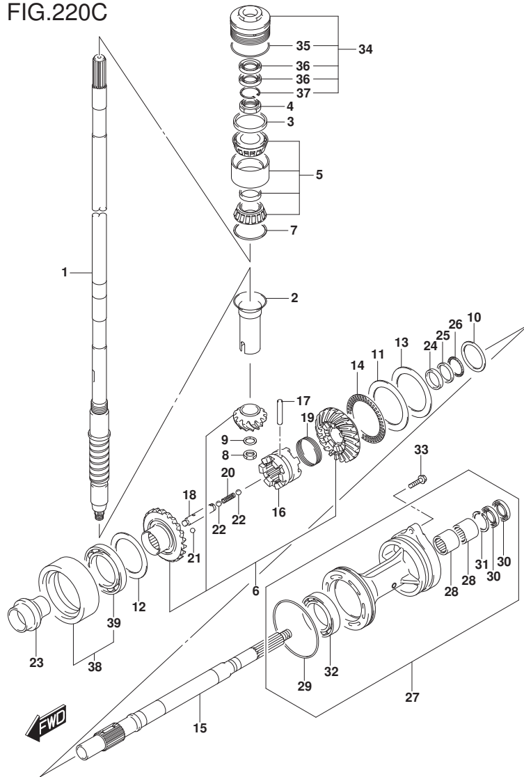
FIG.220C (1-F-14) TRANSMISSION (DF200Z E01)
