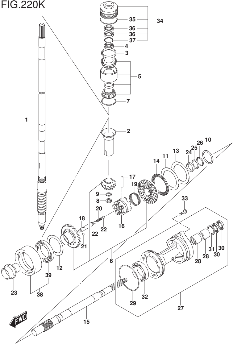
FIG.220K (1-H-8) TRANSMISSION (DF250Z E01)
