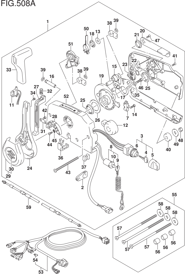
DF250_E01_020_508A OPT:REMOTE CONTROL
