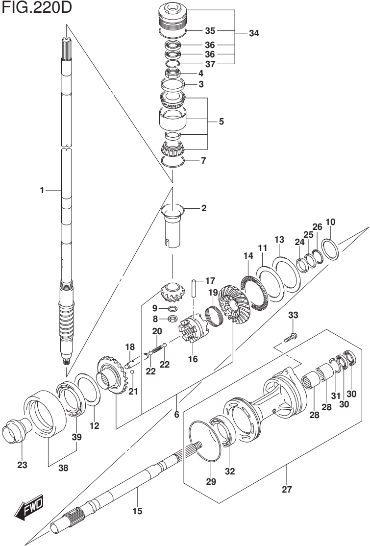
FIG.220D (1-G-5) TRANSMISSION (DF200Z E40)
