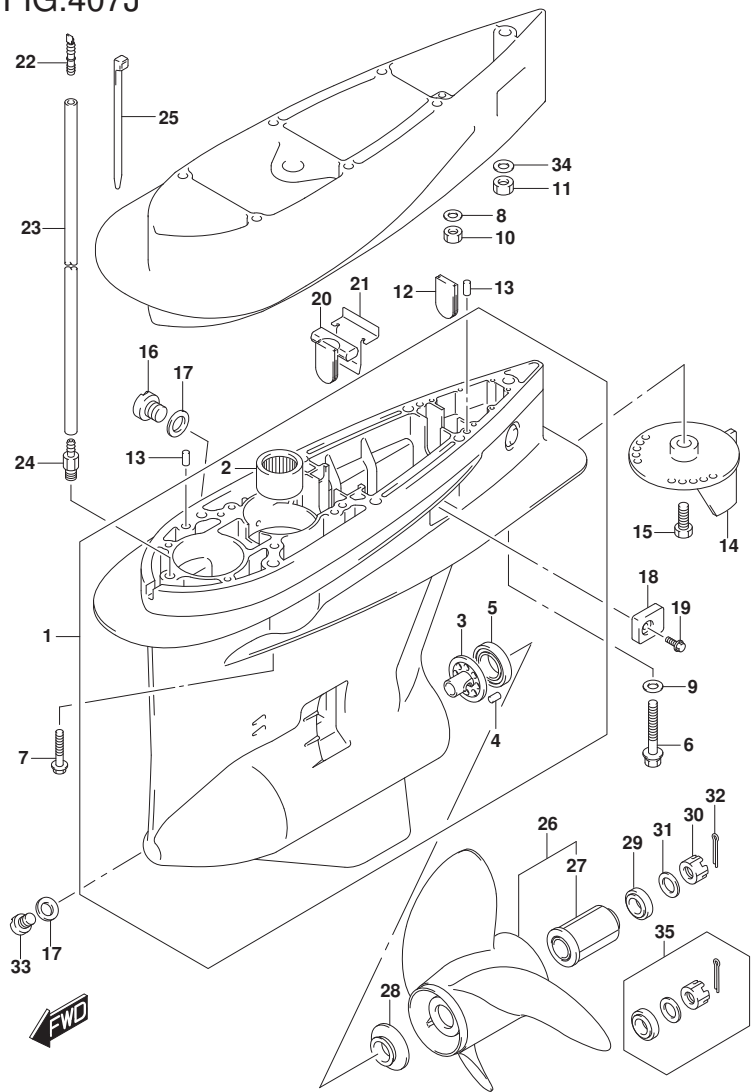
DF250_E01_020_407J GEAR CASE
