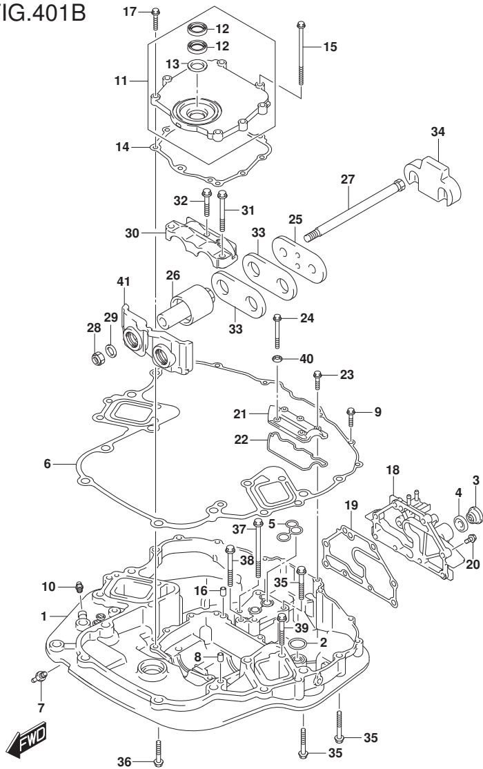
DF250_E01_020_401B ENGINE HOLDER
