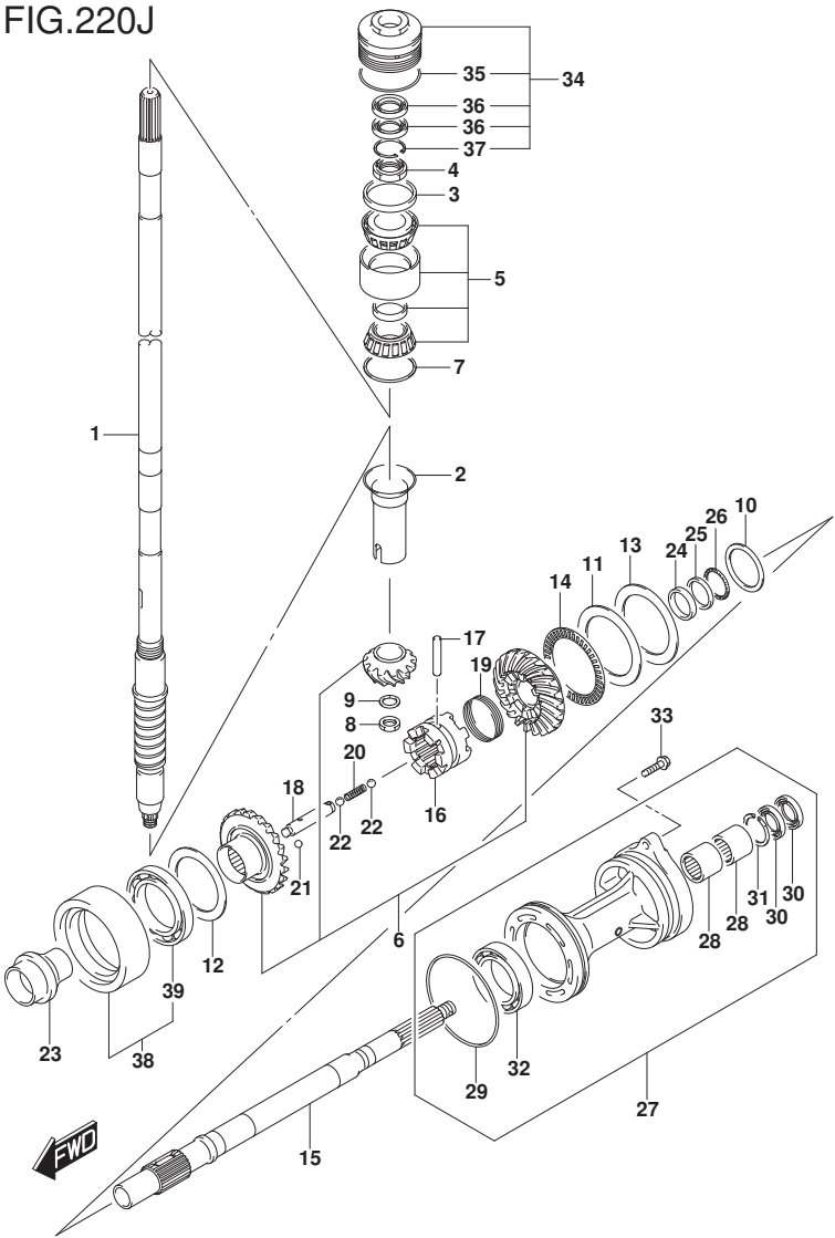
FIG.220J (1-H-5) TRANSMISSION (DF225Z E40)
