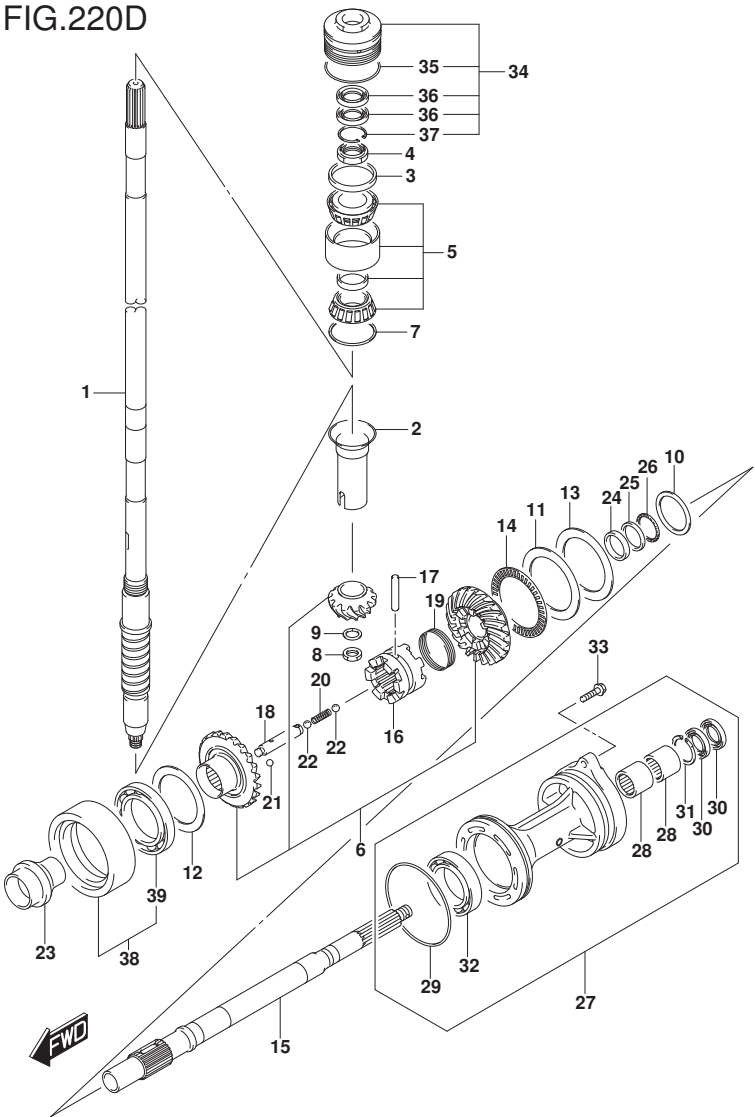
FIG.220D (1-G-3) TRANSMISSION (DF200Z E40)
