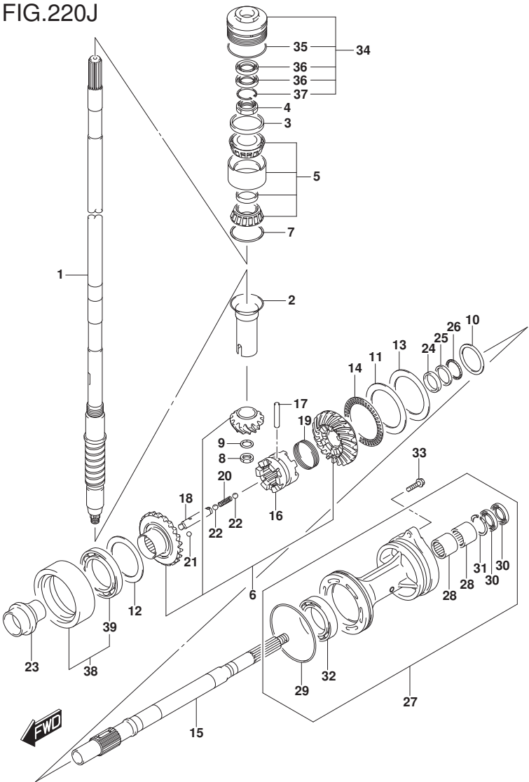
FIG.220J (1-H-6) TRANSMISSION (DF225Z E40)
