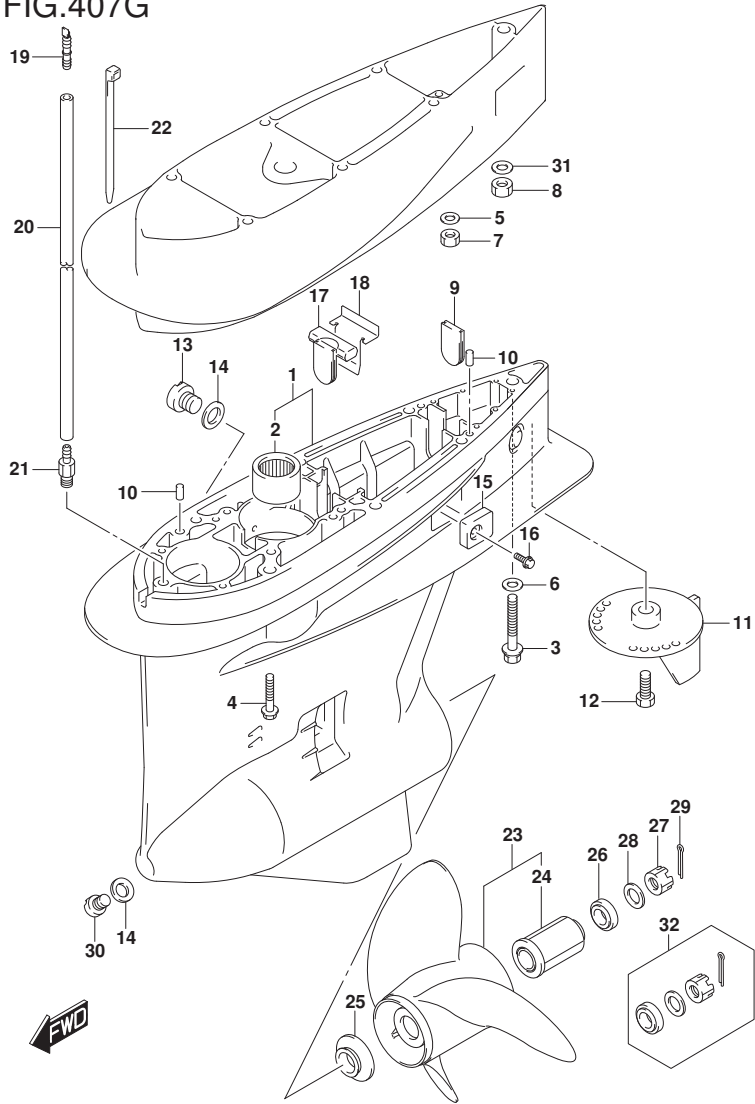
DF250_E01_020_407G GEAR CASE
