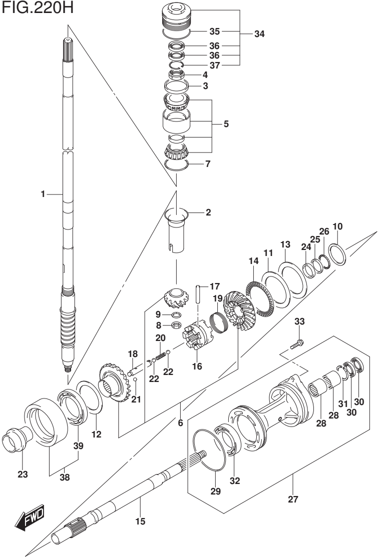
FIG.220H (1-G-15) TRANSMISSION (DF225Z E01)
