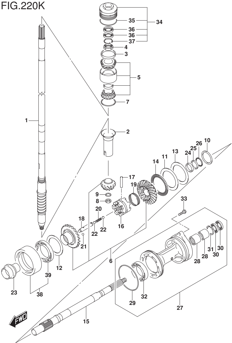
DF250_E01_020_220K TRANSMISSION
