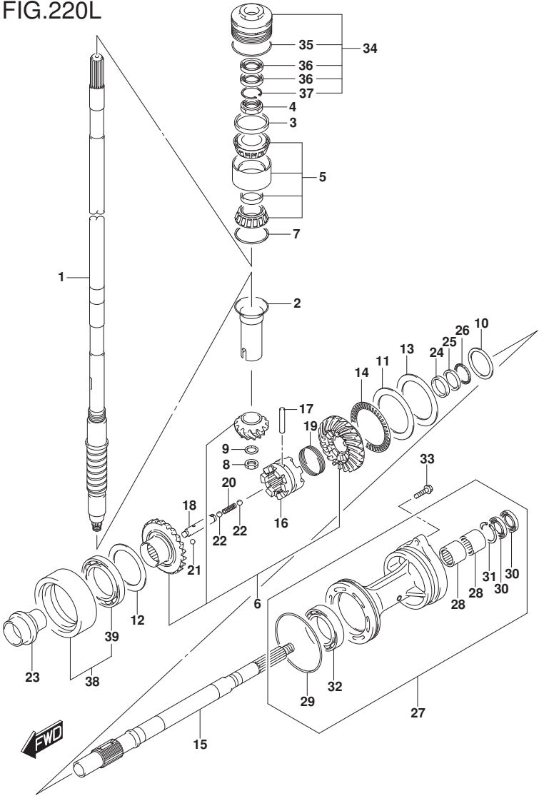
FIG.220L (1-H-12) TRANSMISSION (DF250Z E40)
