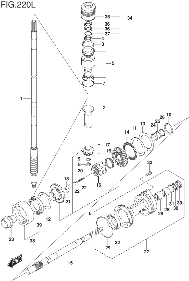
FIG.220L (1-H-11) TRANSMISSION (DF250Z E40)
