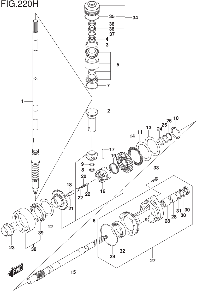
FIG.220H (1-H-2) TRANSMISSION (DF225Z E01)
