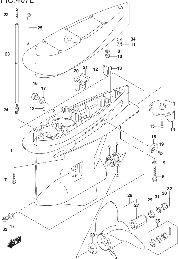
DF250_E01_020_407L GEAR CASE
