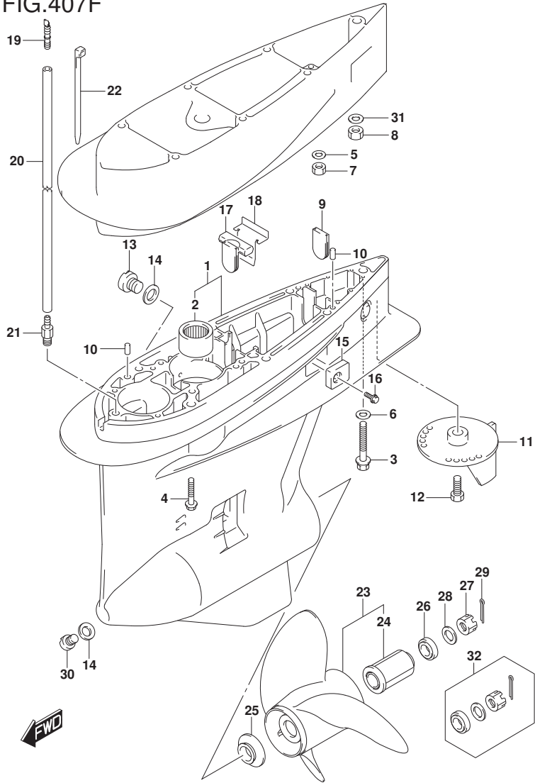
DF250_E01_020_407F GEAR CASE
