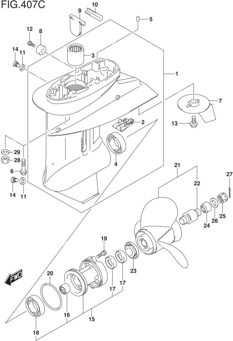
FIG.407C (1-H-2) GEAR CASE (DF30AQ)
