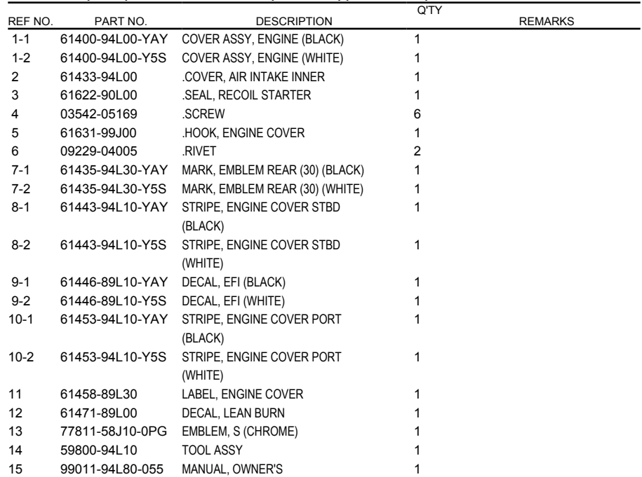
FIG.420E (1-I-4) ENGINE COVER (DF30AT)(DF30ATH)
