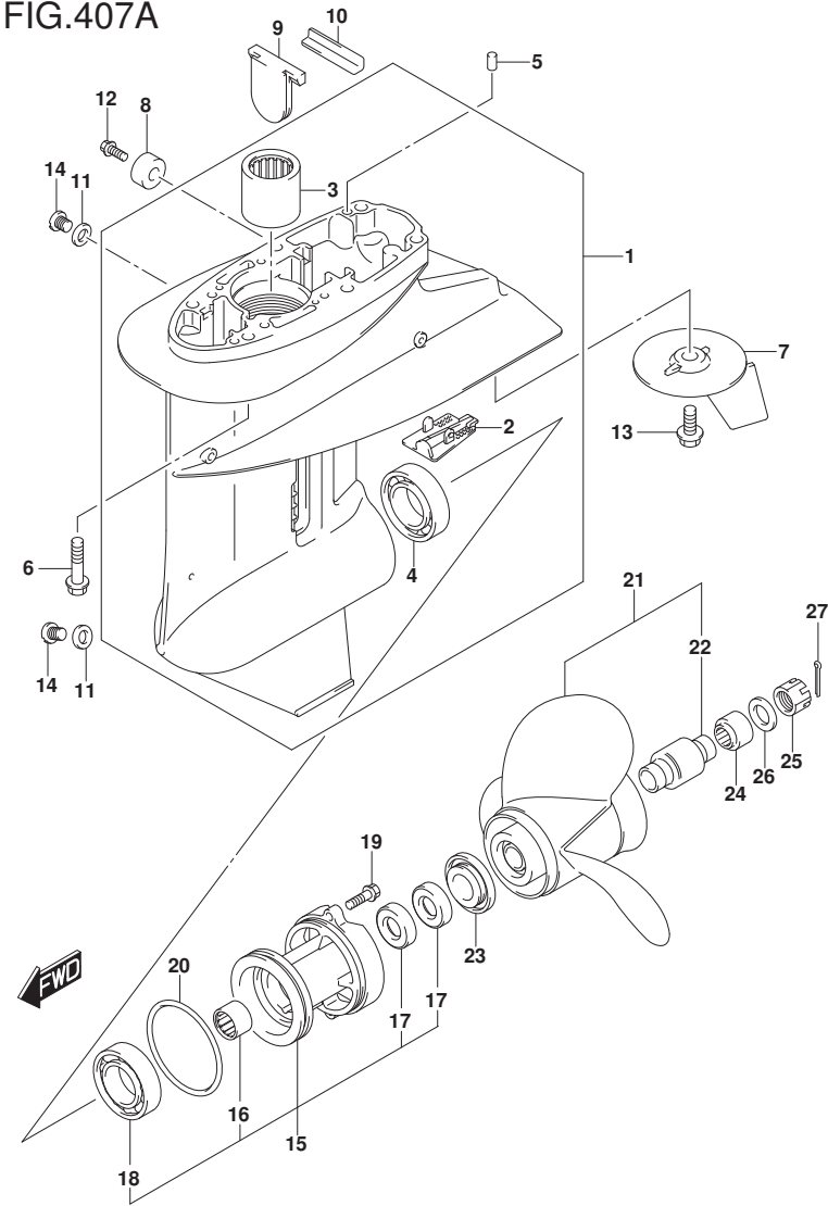
FIG.407A (1-G-12) GEAR CASE (DF25A)(DF30AR)
