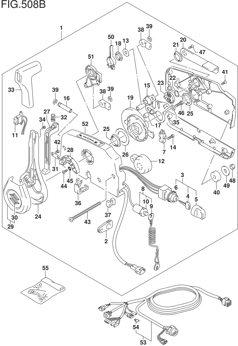
FIG.508B (1-J-9) OPT:REMOTE CONTROL (DF25ATH)(DF30ATH)
