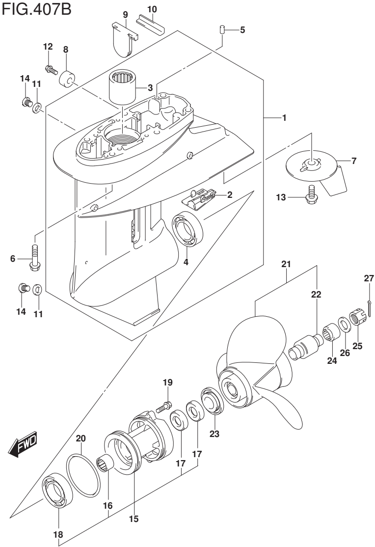
FIG.407B (1-G-15) GEAR CASE (DF25AT)(DF25ATH)(DF30A)(DF30AT)(DF30ATH)
