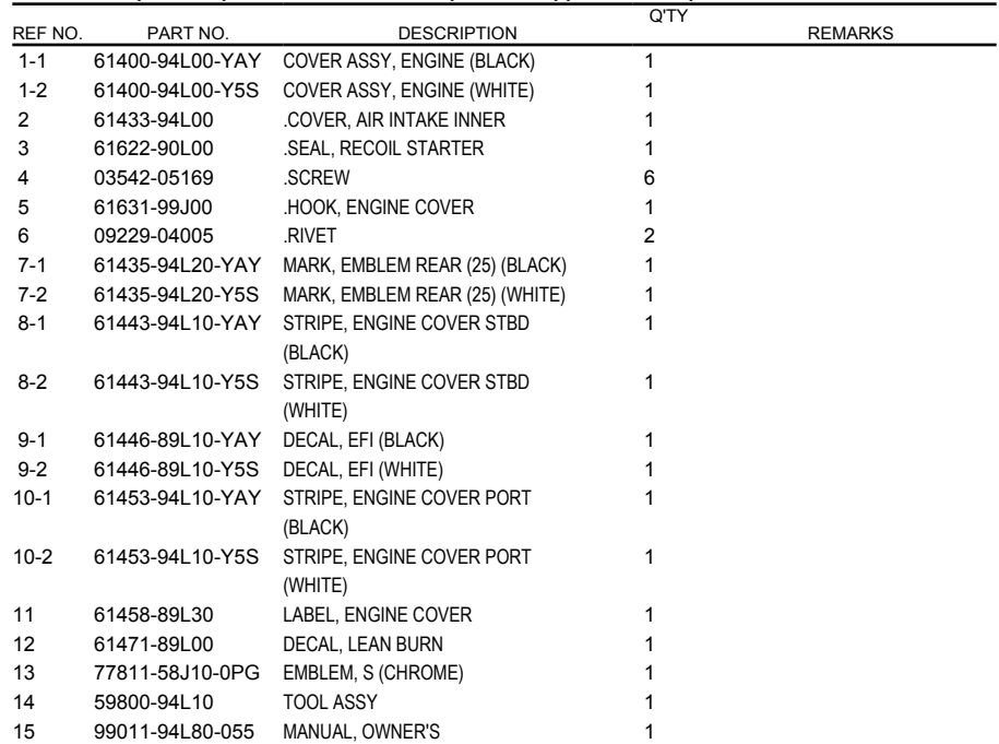
FIG.420B (1-H-15) ENGINE COVER (DF25AT)(DF25ATH)
