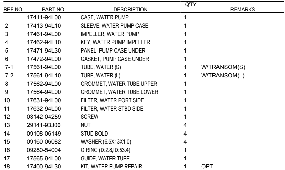
FIG.160B (1-C-3) WATER PUMP (DF30A)
