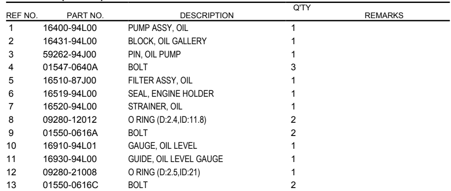
FIG.175A (1-C-10) OIL PUMP
