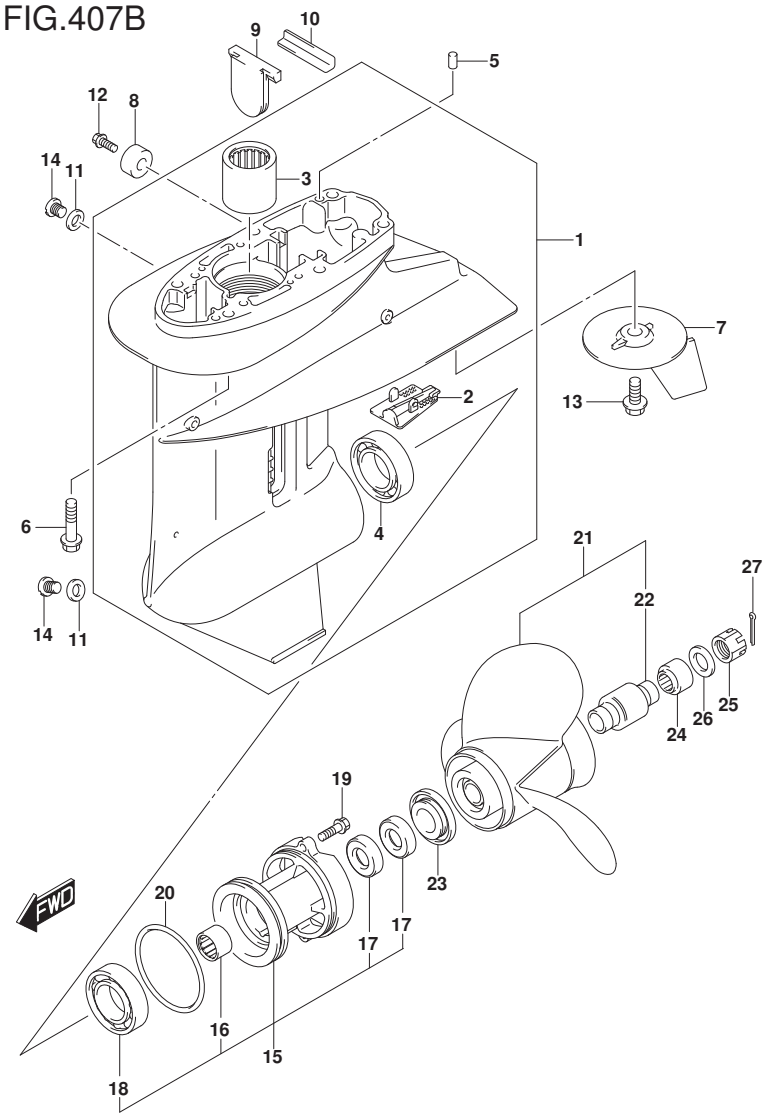
FIG.407B (1-G-14) GEAR CASE (DF25AT)(DF25ATH)(DF30A)(DF30AT)(DF30ATH)
