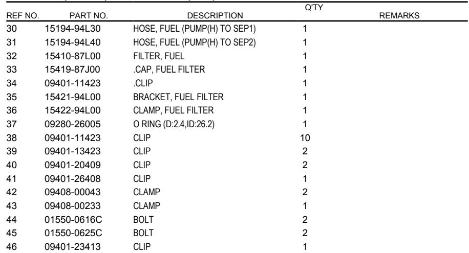
FIG.146B (1-B-15) FUEL PUMP (P40)
