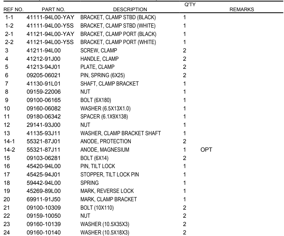
FIG.335C (1-F-4) CLAMP BRACKET (DF30A)
