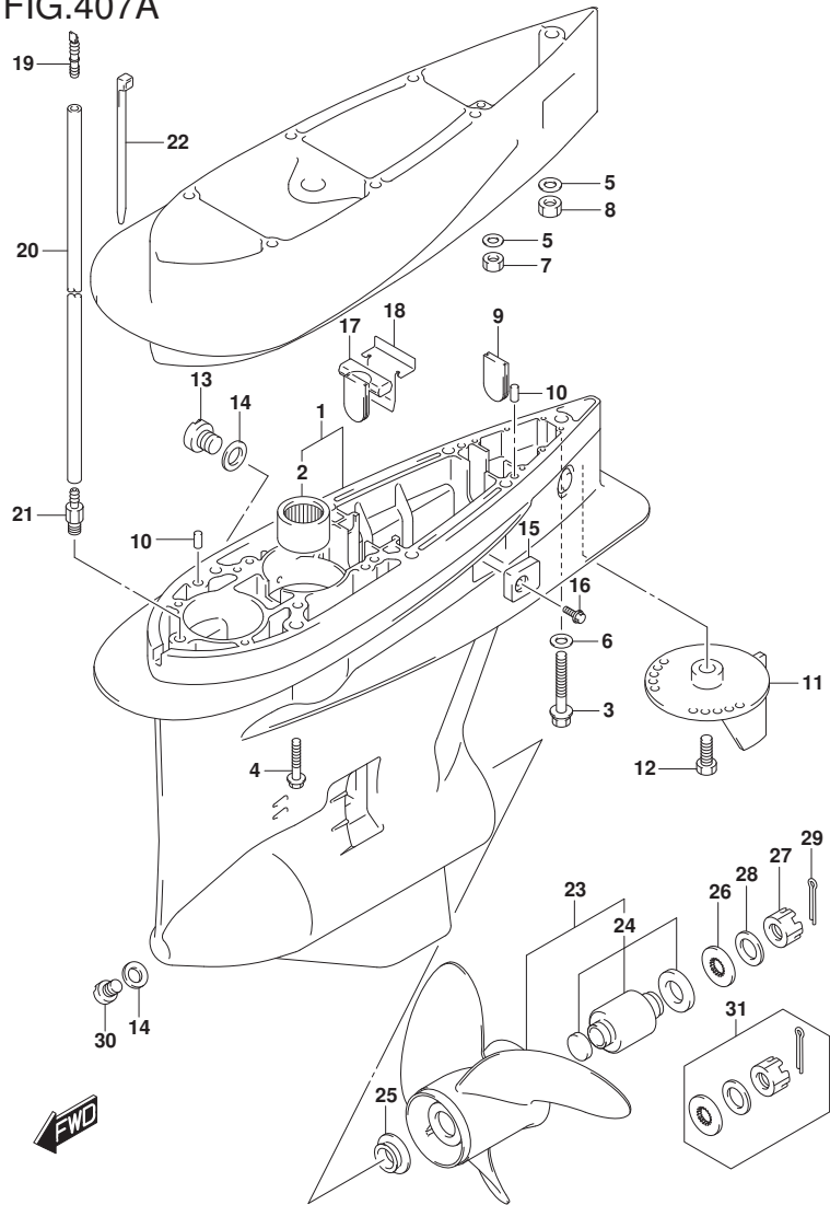
DF250_E01_018_407A GEAR CASE
