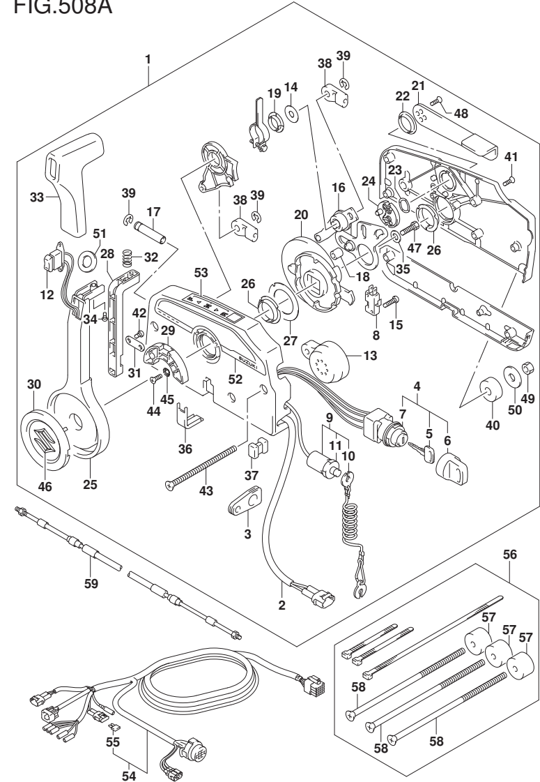
DF250_E01_018_508A OPT:REMOTE CONTROL
