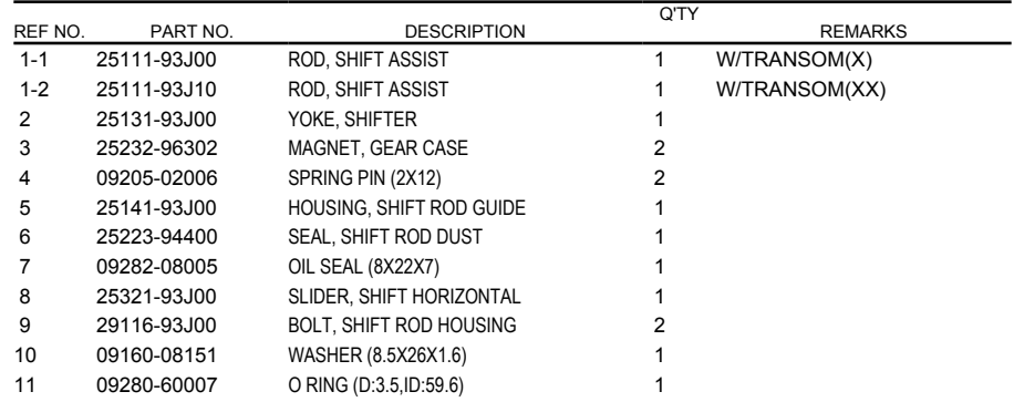
FIG.206B (1-E-11) CLUTCH ROD (DF200Z E01)
