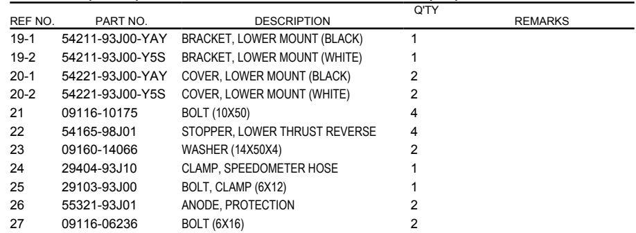
FIG.405C (1-I-12) DRIVE SHAFT HOUSING TRANSOM(XX)
