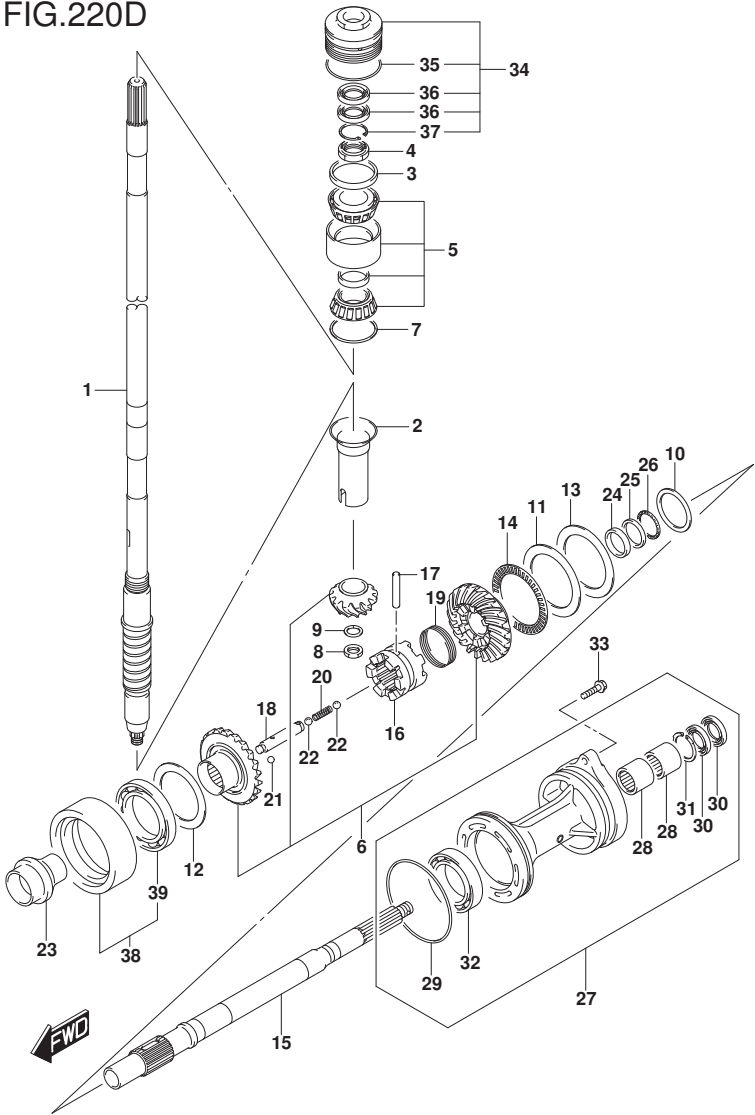
FIG.220D (1-F-12) TRANSMISSION (DF200Z E40)
