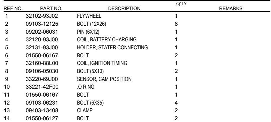
FIG.303A (1-G-6) MAGNETO (DF200T)(DF200Z)(DF225T)(DF225Z)
