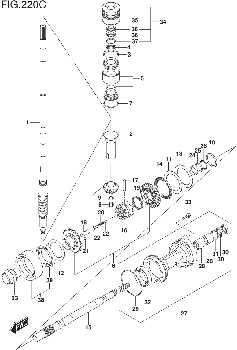
FIG.220C (1-F-7) TRANSMISSION (DF200Z E01)
