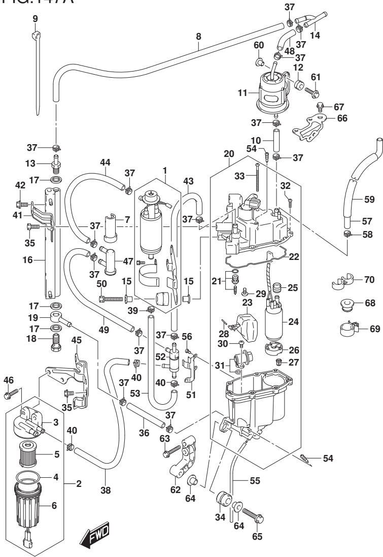
DF250_E01_018_147A FUEL PUMP/FUEL VAPOR SEPARATOR
