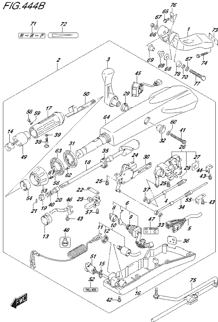
FIG.444B (2-I-9) TILLER HANDLE (DF70ATH E40)
