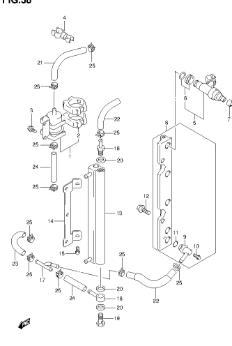
DF80A E01 013_008 FUEL INJECTOR
