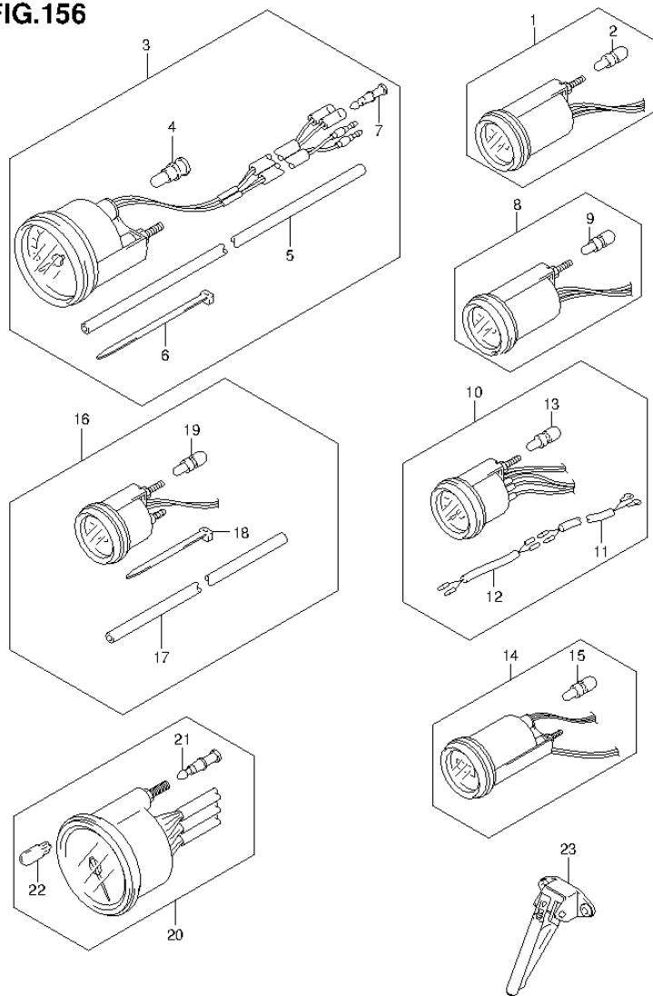
FIG.156 (2-E-3) OPT:METER (DF90ATH E40)
