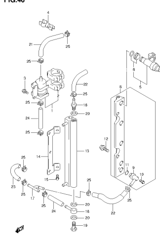
DF80A E01 013_040 FUEL INJECTOR
