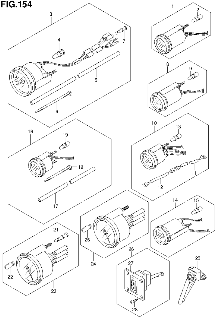
FIG.154 (2-D-13) OPT:METER (DF90A E40)
