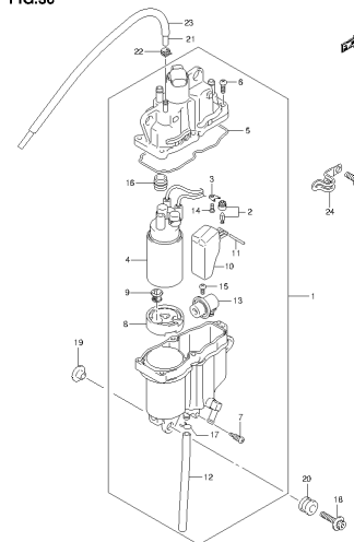
DF80A E01 013_006 FUEL VAPOR SEPARATOR
