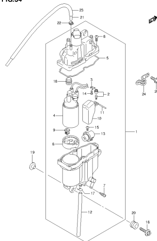
DF80A E01 013_004 FUEL VAPOR SEPARATOR
