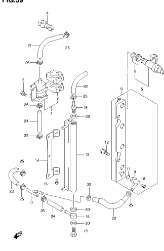
DF80A E01 013_009 FUEL INJECTOR
