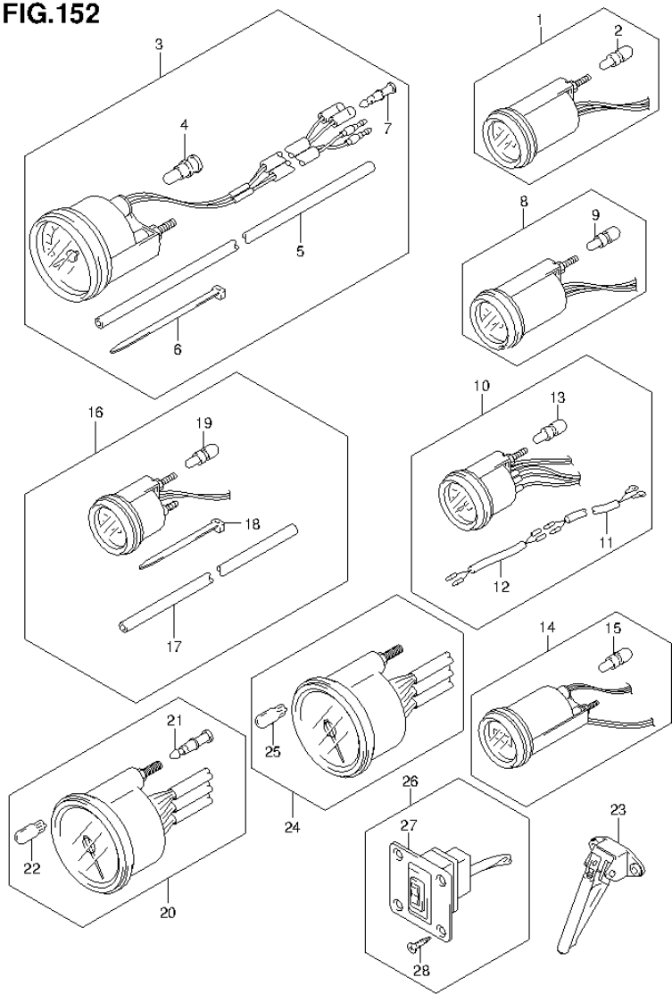
FIG.152 (2-D-9) OPT:METER (DF80A E40)
