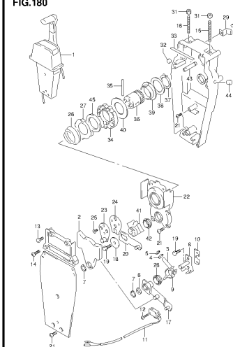
DF80A E01 013_180 OPT REMOTE CONTROL ASSY SINGLE (2)
