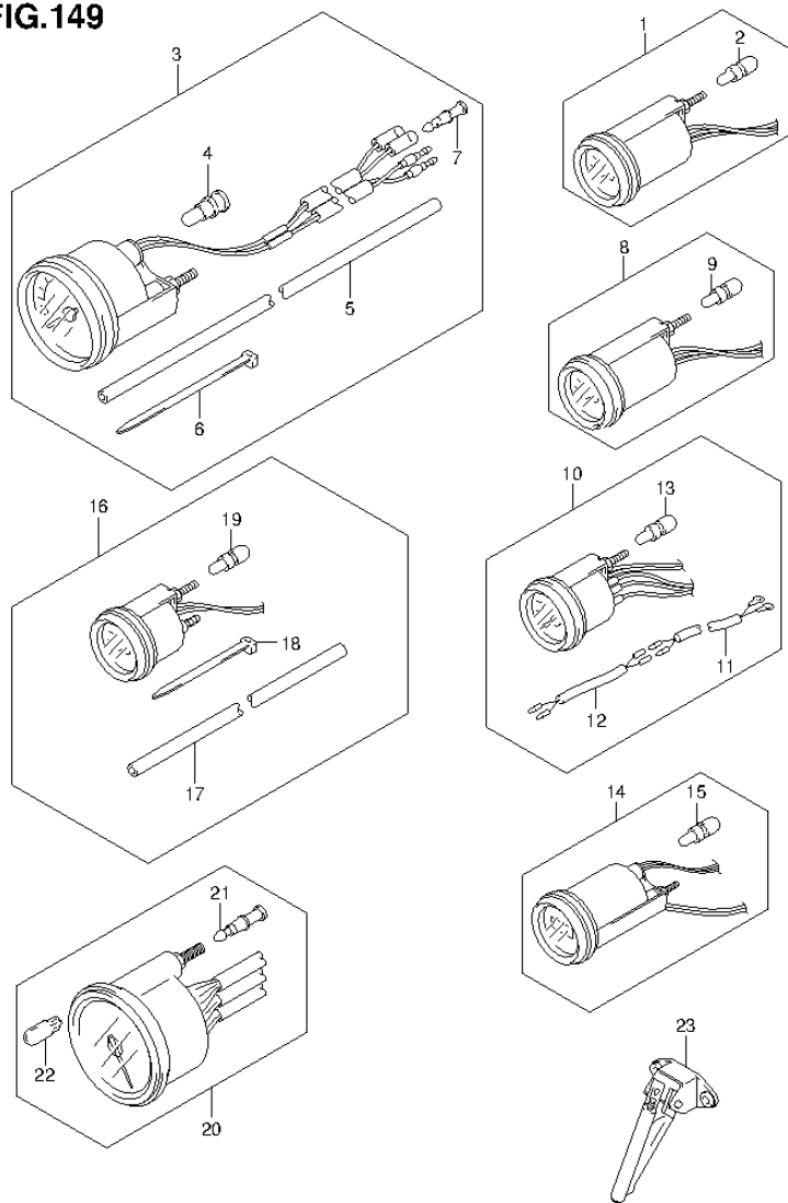
FIG.149 (2-D-2) OPT:METER (DF70ATH E1)
