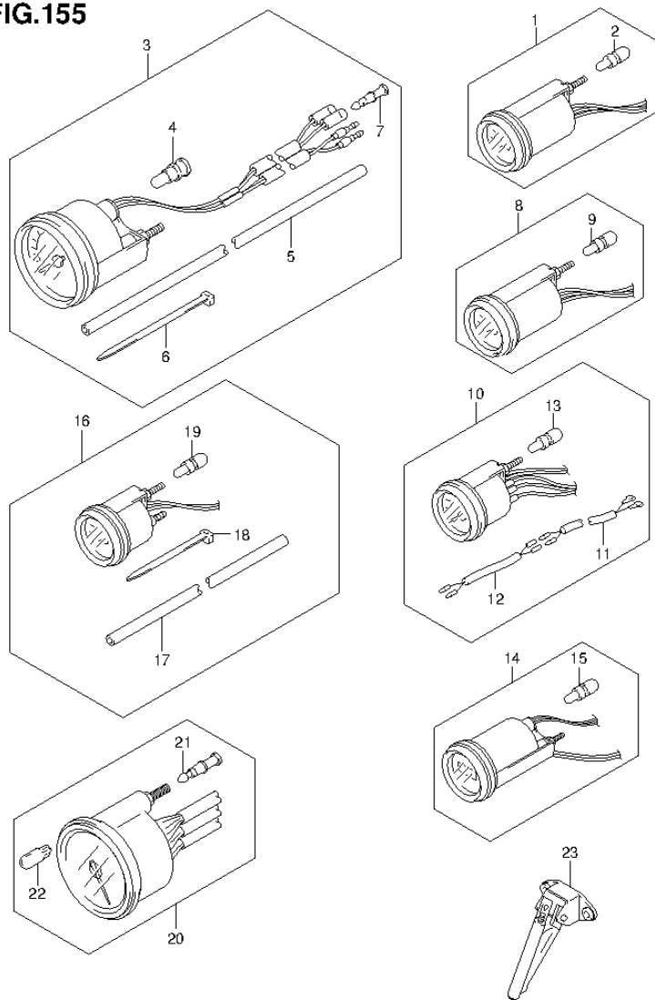
FIG.155 (2-D-15) OPT:METER (DF90ATH E1)
