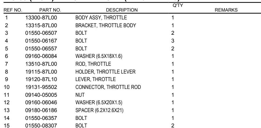
FIG.63 (1-G-4) THROTTLE BODY (DF70ATH E40)
