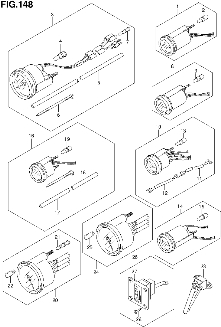
FIG.148 (2-C-15) OPT:METER (DF70A E40)
