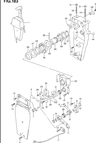
DF80A E01 013_183 OPT REMOTE CONTROL ASSY SINGLE (2)
