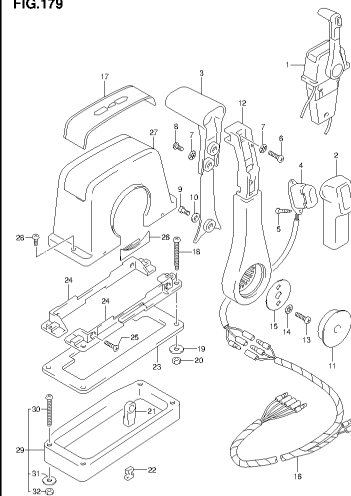
DF80A E01 013_179 OPT REMOTE CONTROL ASSY SINGLE (1)
