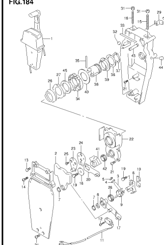
DF80A E01 013_184 OPT REMOTE CONTROL ASSY SINGLE (2)
