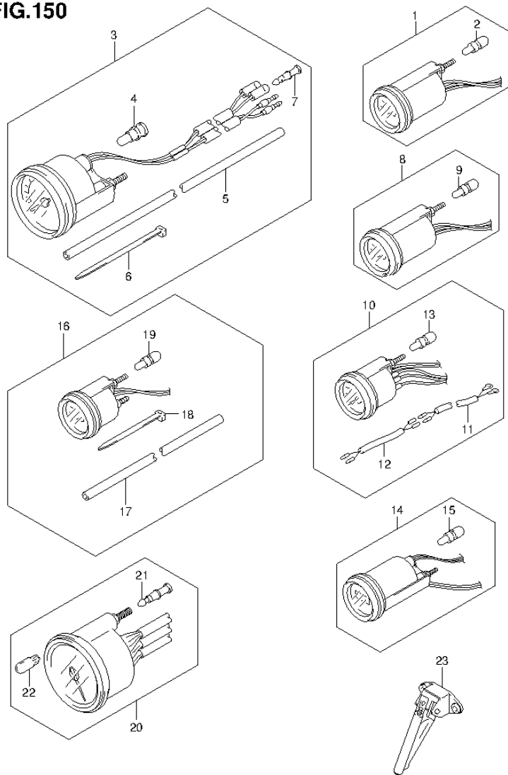
FIG.150 (2-D-5) OPT:METER (DF70ATH E40)
