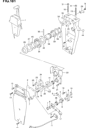
DF80A E01 013_181 OPT REMOTE CONTROL ASSY SINGLE (2)
