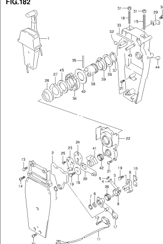
DF80A E01 013_182 OPT REMOTE CONTROL ASSY SINGLE (2)
