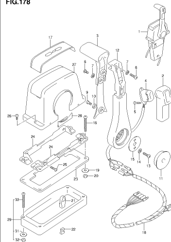
DF80A E01 013_178 OPT REMOTE CONTROL ASSY SINGLE (1)
