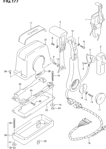
DF80A E01 013_177 OPT REMOTE CONTROL ASSY SINGLE (1)
