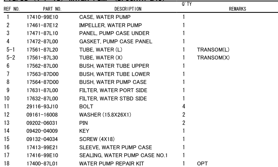
FIG. 58 (1-F-13) WATER PUMP (DF90ATH E40)
