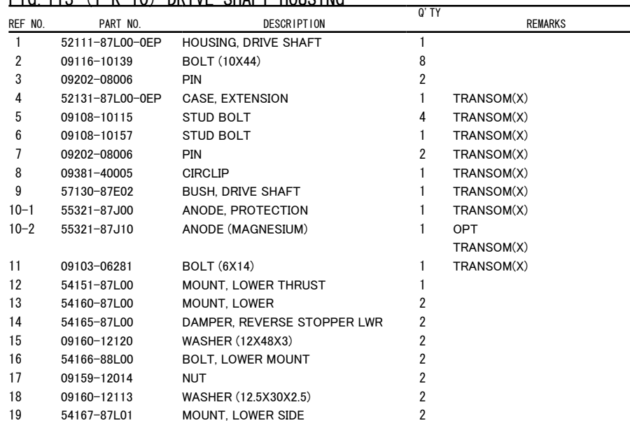
FIG. 113 (1-K-10) DRIVE SHAFT HOUSING
