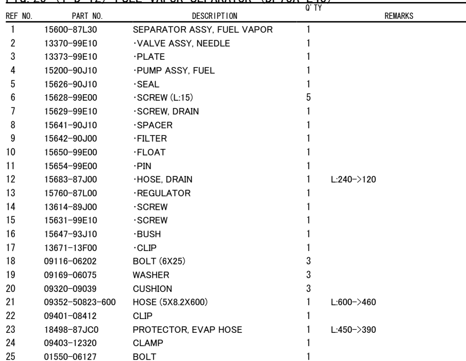
FIG. 29 (1-D-12) FUEL VAPOR SEPARATOR (DF70A E40)
