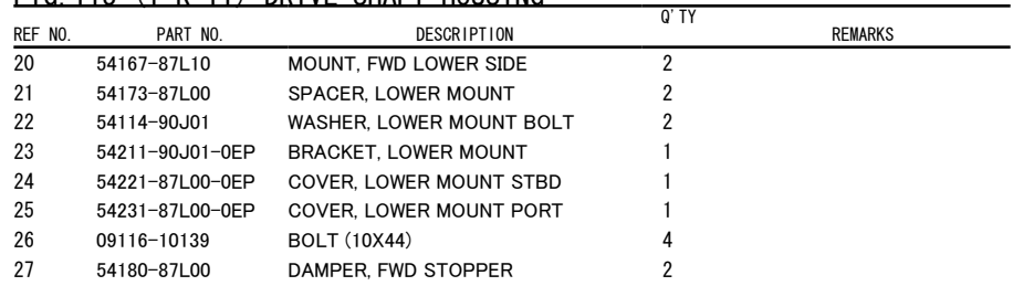
FIG. 113 (1-K-11) DRIVE SHAFT HOUSING
