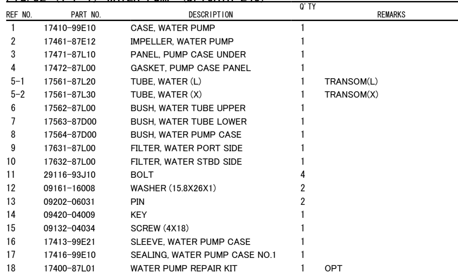
FIG. 52 (1-F-7) WATER PUMP (DF70ATH E40)
