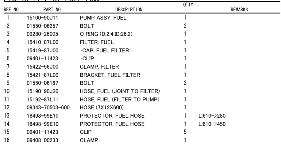
FIG. 48 (1-F-3) FUEL PUMP
