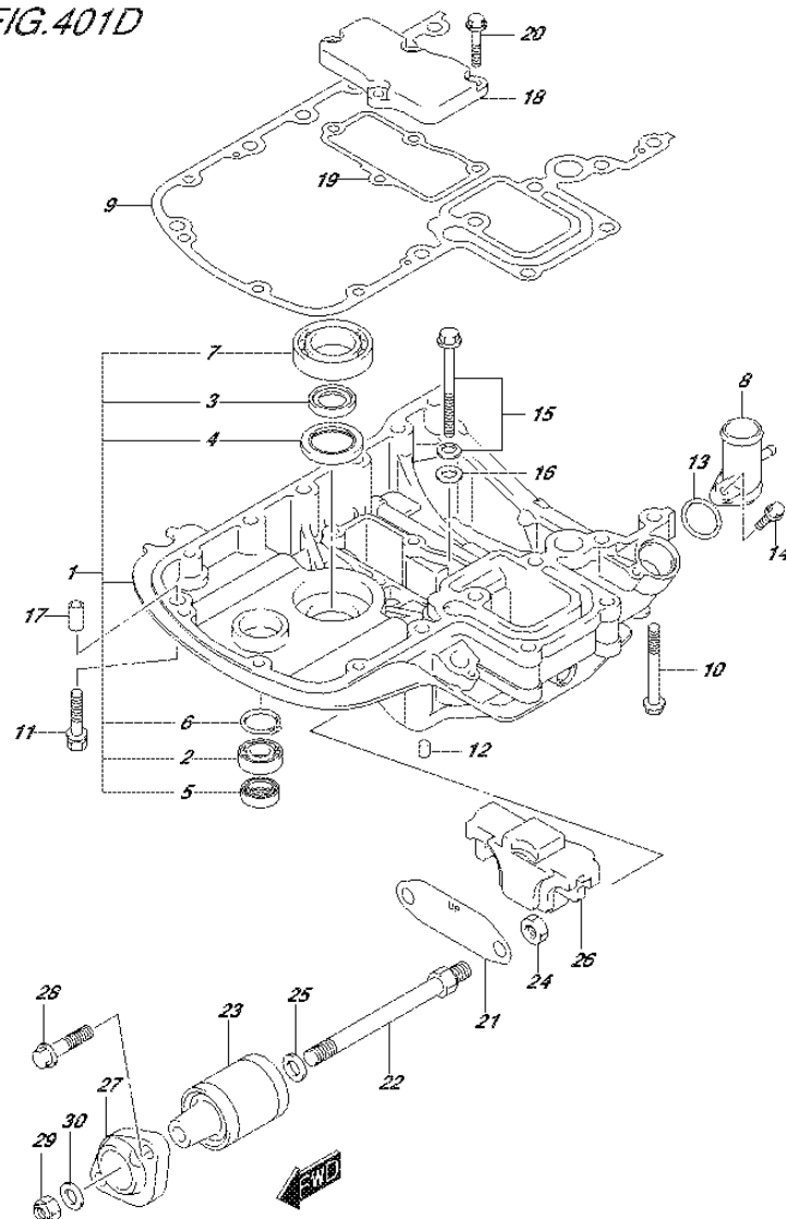
FIG.401D (2-F-9) ENGINE HOLDER (DF115AZ E11)
