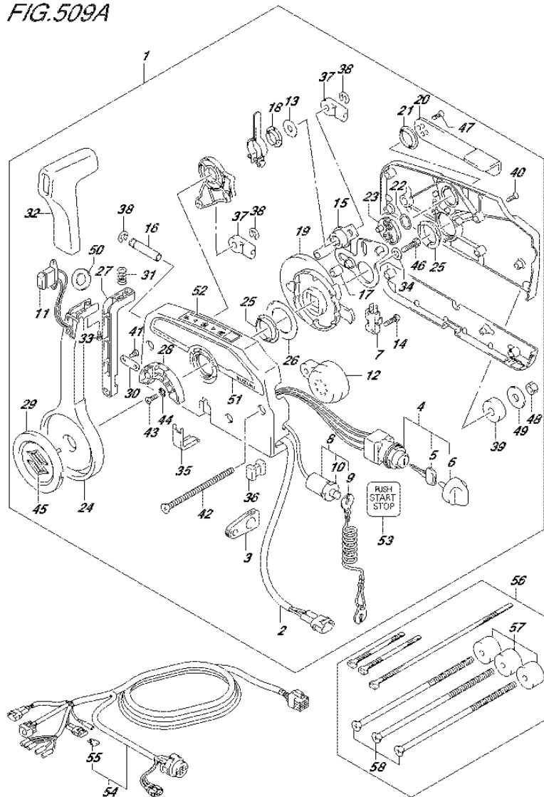
FIG.509A (3-C-7) OPT:REMOTE CONTROL (1) (DF100AT E11)
