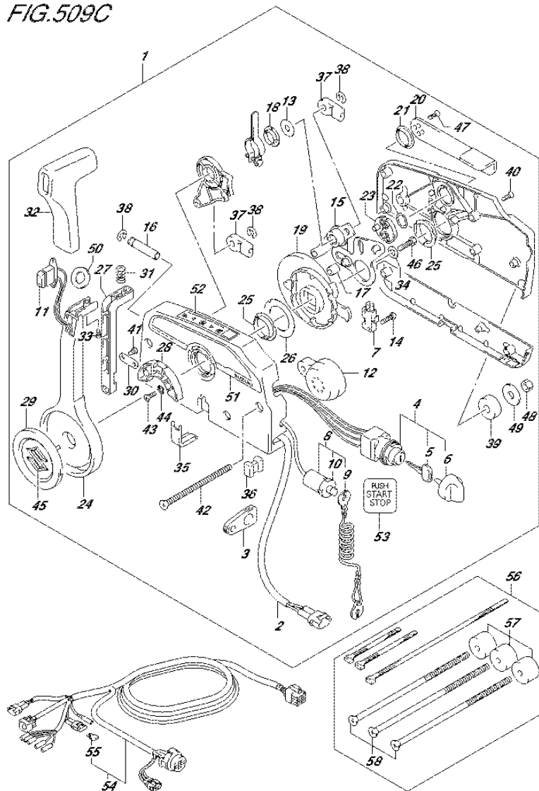
FIG.509C (3-C-13) OPT:REMOTE CONTROL (1) (DF115AZ E11)
