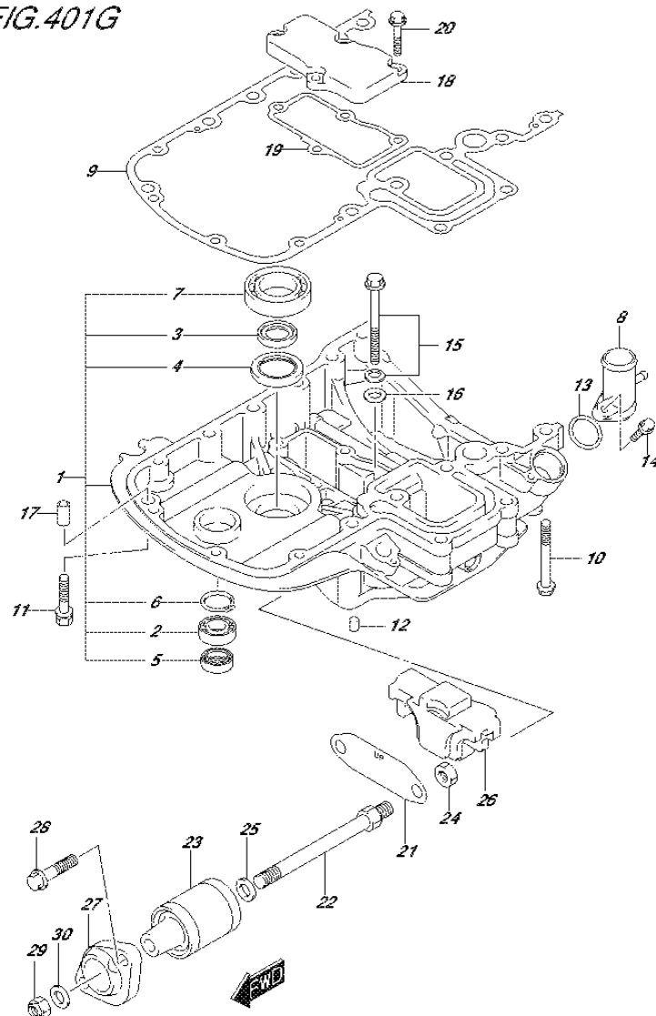
FIG.401G (2-F-12) ENGINE HOLDER (DF140AT E40)
