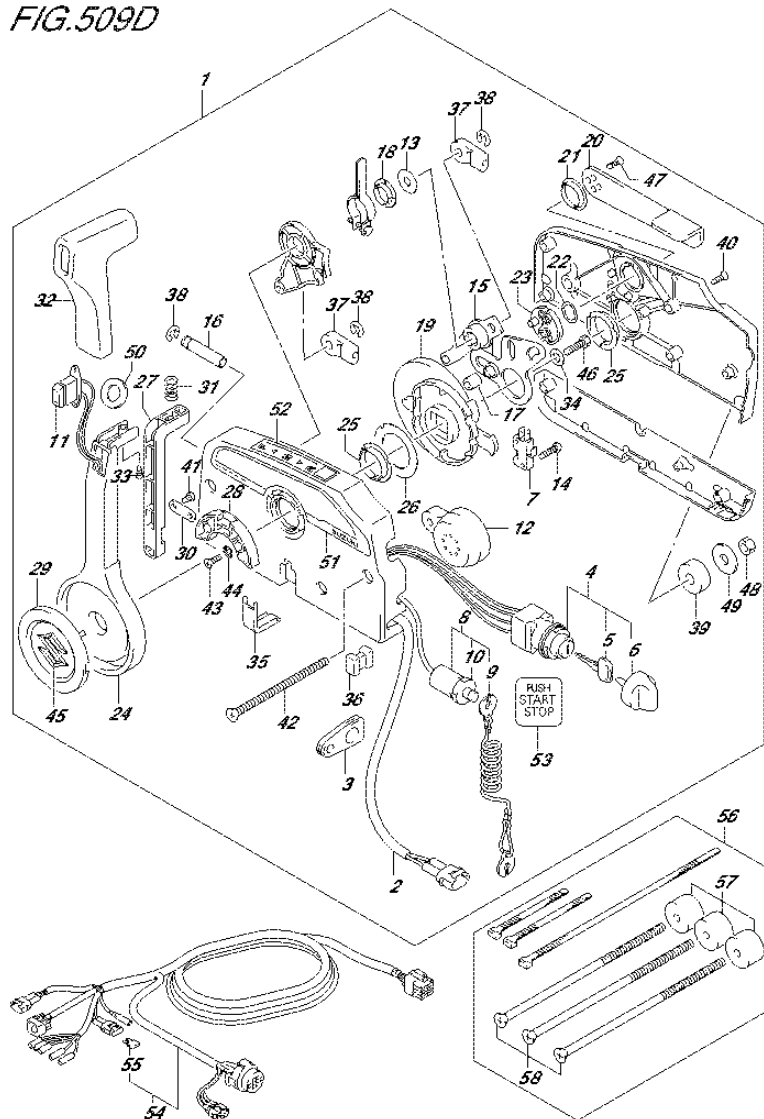
FIG.509D (3-C-15) OPT:REMOTE CONTROL (1) (DF140AT E11)
