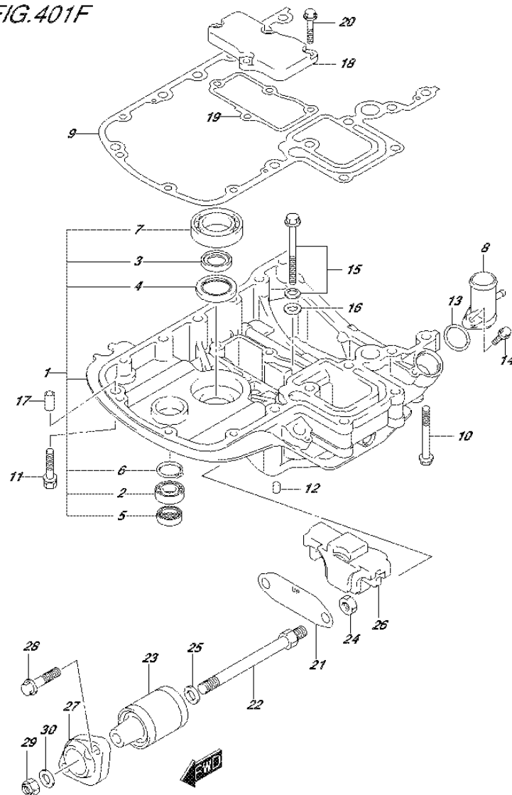
FIG.401F (2-F-11) ENGINE HOLDER (DF140AT E11)
