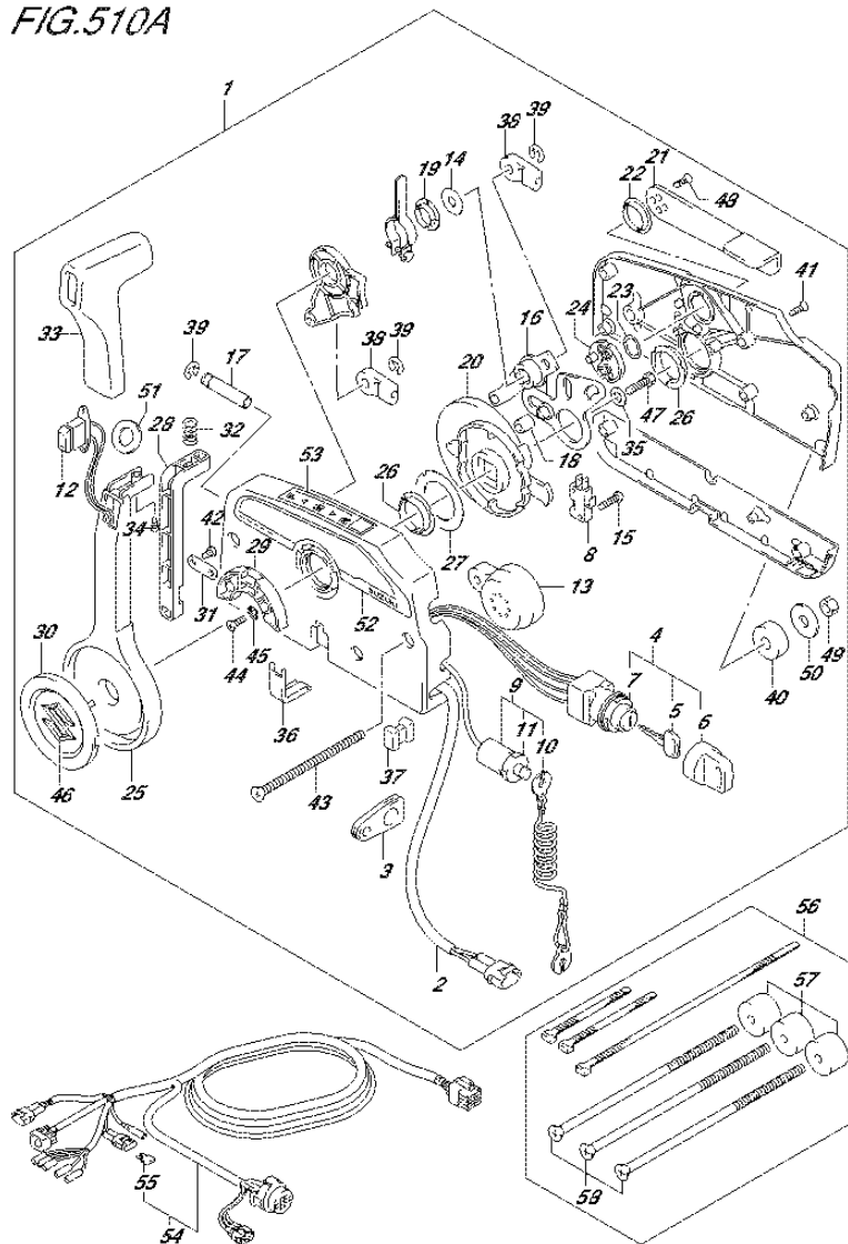
FIG.510A (3-D-7) OPT:REMOTE CONTROL (2) (DF100AT E11)
