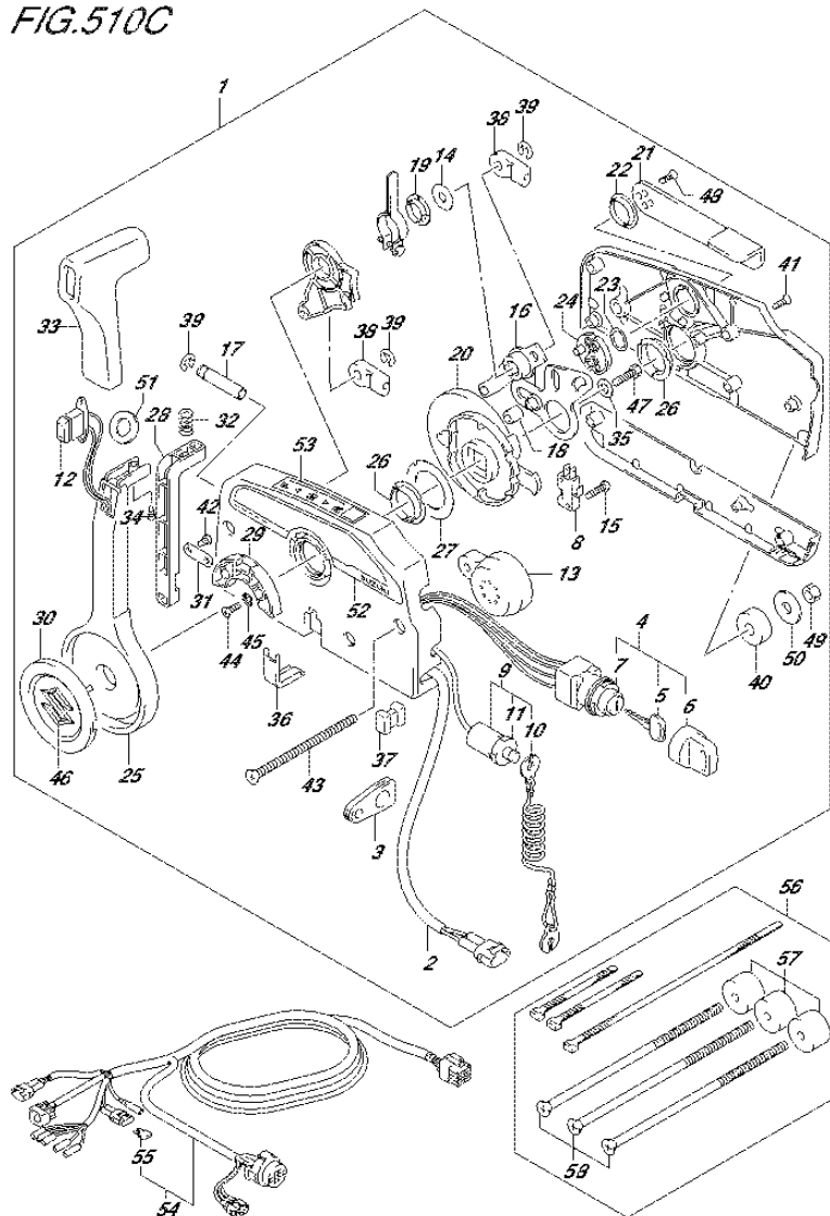
FIG.510C (3-D-12) OPT:REMOTE CONTROL (2) (DF115AT E40)
