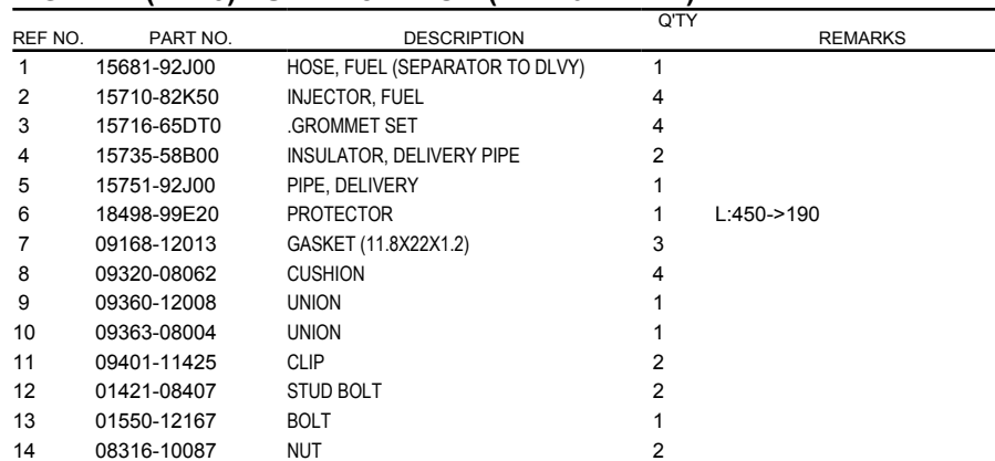
FIG.144F (1-E-3) FUEL INJECTOR (DF140AT E11)
