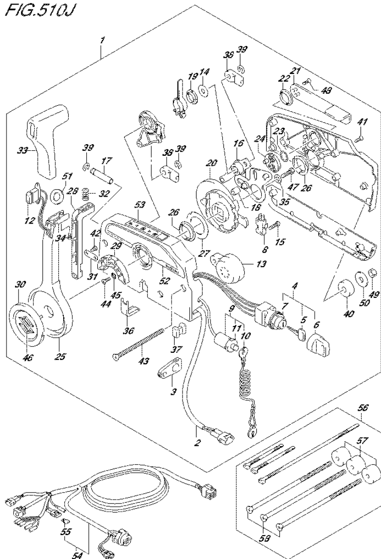
FIG.510J (3-F-3) OPT:REMOTE CONTROL (2) (DF140AZ E40)
