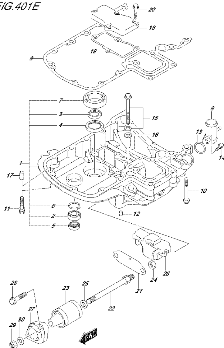
FIG.401E (2-F-10) ENGINE HOLDER (DF115AZ E40)
