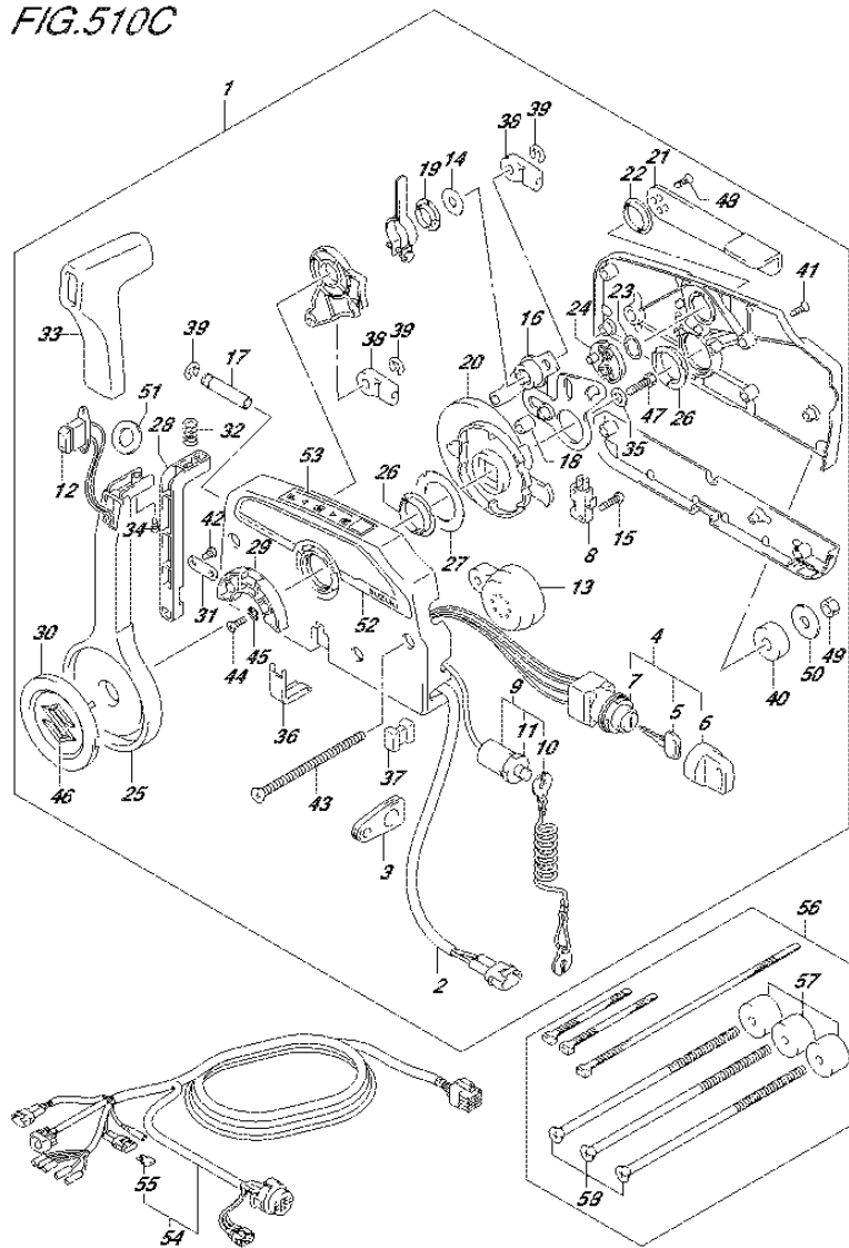
FIG.510C (3-D-13) OPT:REMOTE CONTROL (2) (DF115AT E40)
