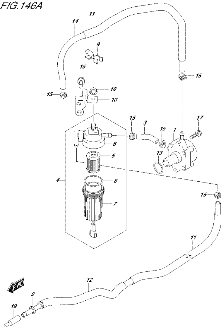
FIG.146A (1-E-8) FUEL PUMP
