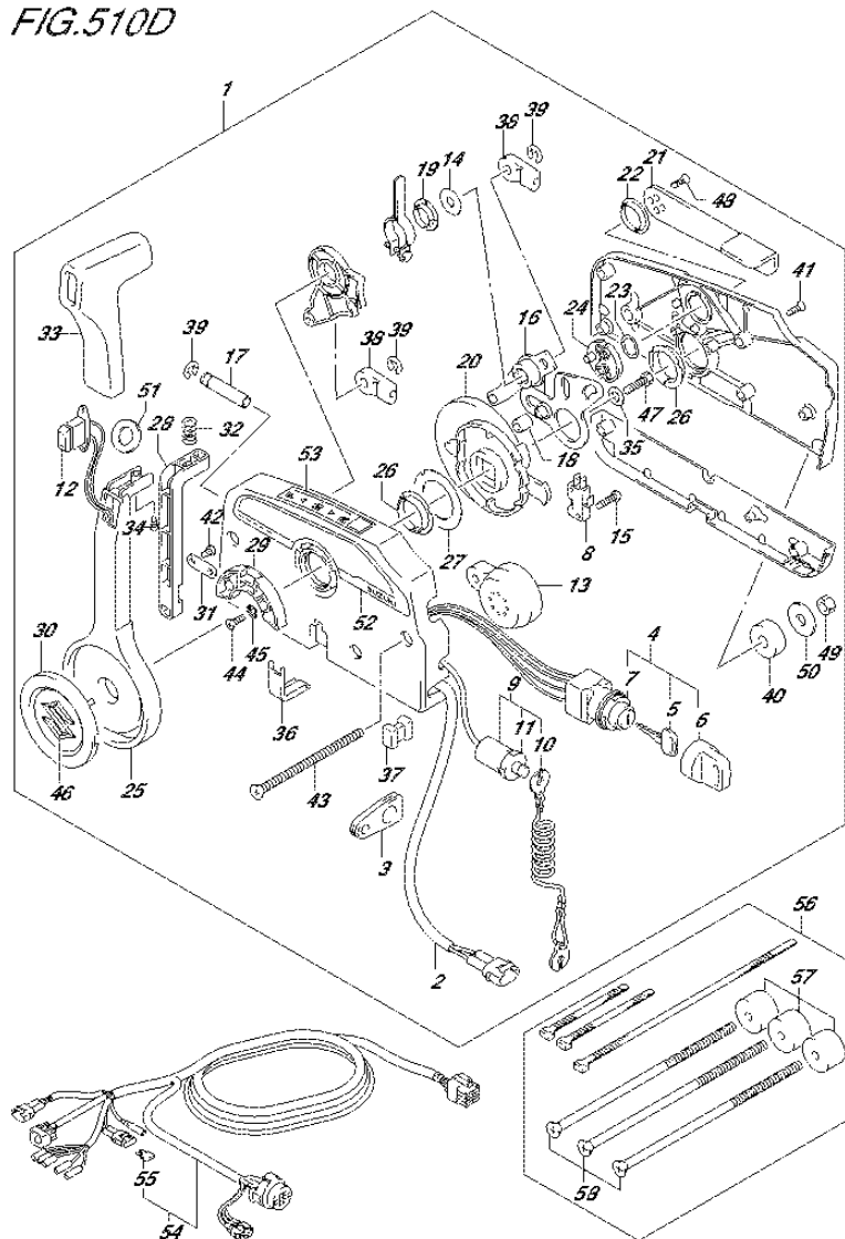
FIG.510D (3-E-2) OPT:REMOTE CONTROL (2) (DF115AZ E11)
