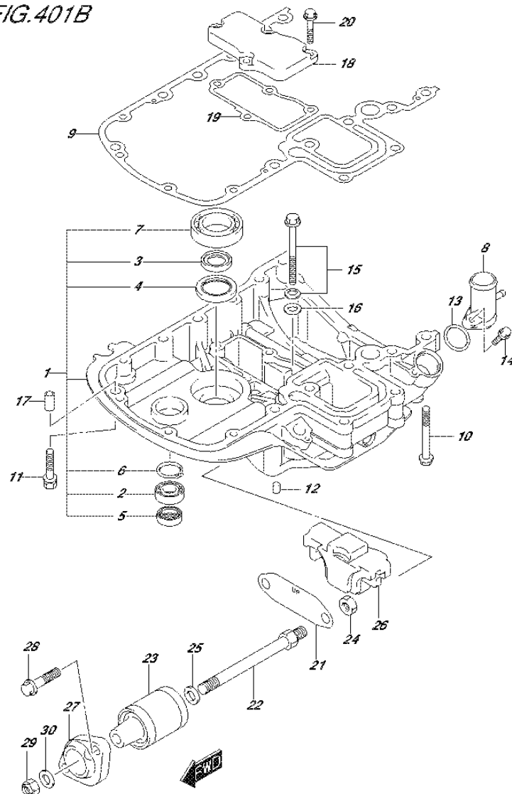
FIG.401B (2-F-7) ENGINE HOLDER (DF115AT E11)
