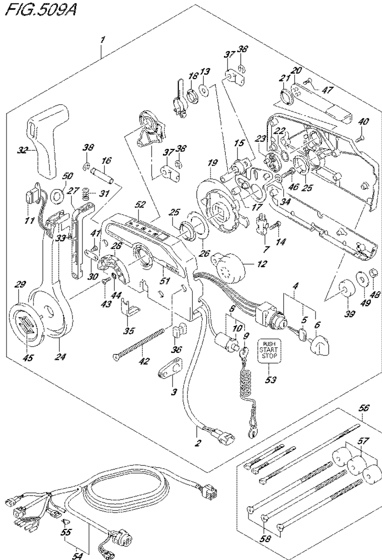
FIG.509A (3-C-5) OPT:REMOTE CONTROL (1) (DF100AT E11)
