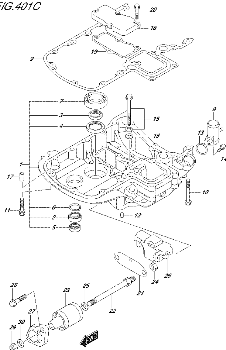
FIG.401C (2-F-8) ENGINE HOLDER (DF115AT E40)
