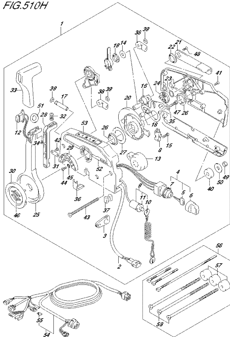
FIG.510H (3-E-15) OPT:REMOTE CONTROL (2) (DF140AZ E11)
