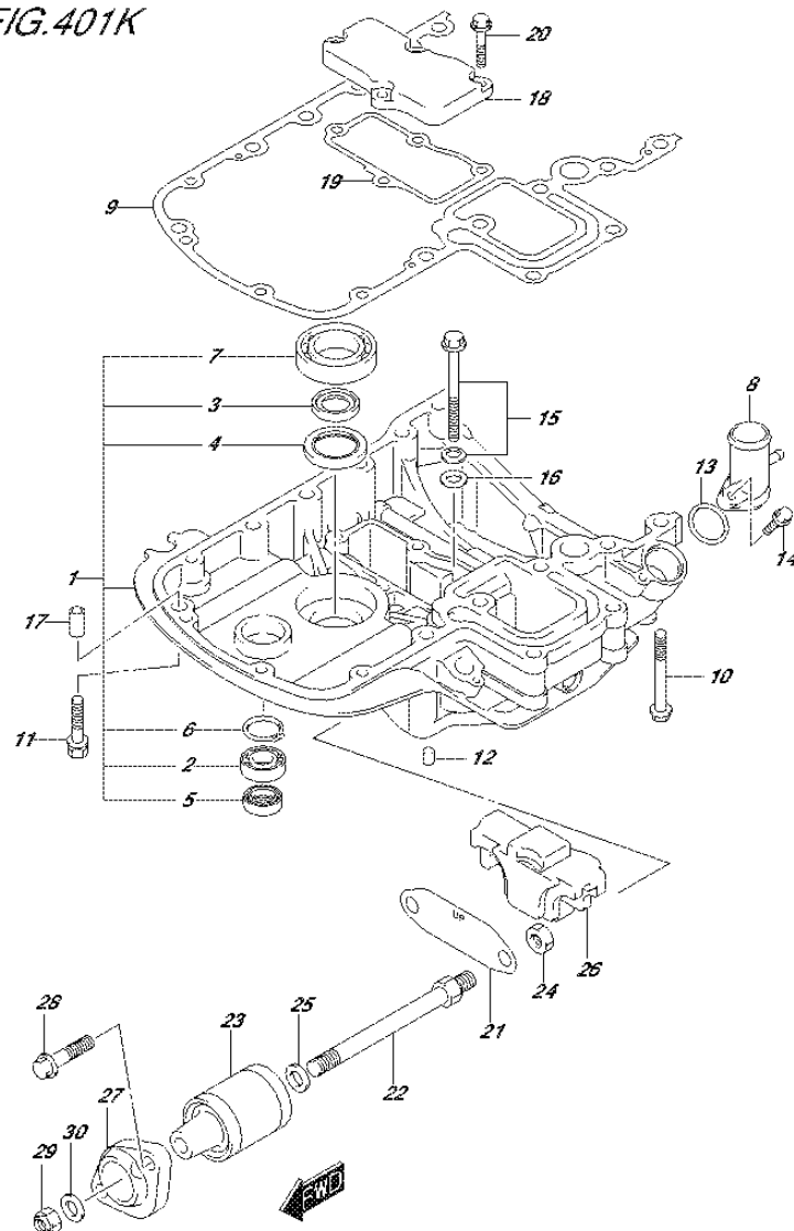
FIG.401K (2-F-15) ENGINE HOLDER (DF115AST E03)
