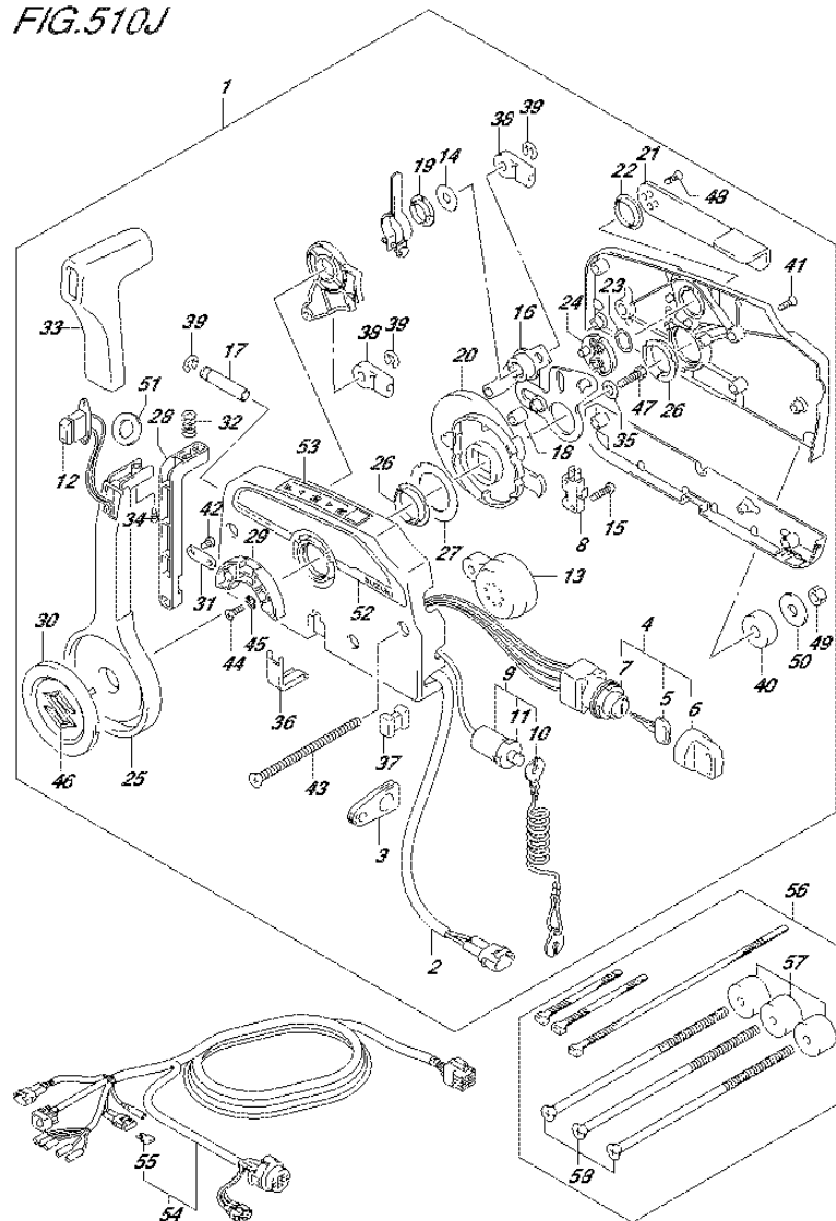
FIG.510J (3-F-4) OPT:REMOTE CONTROL (2) (DF140AZ E40)
