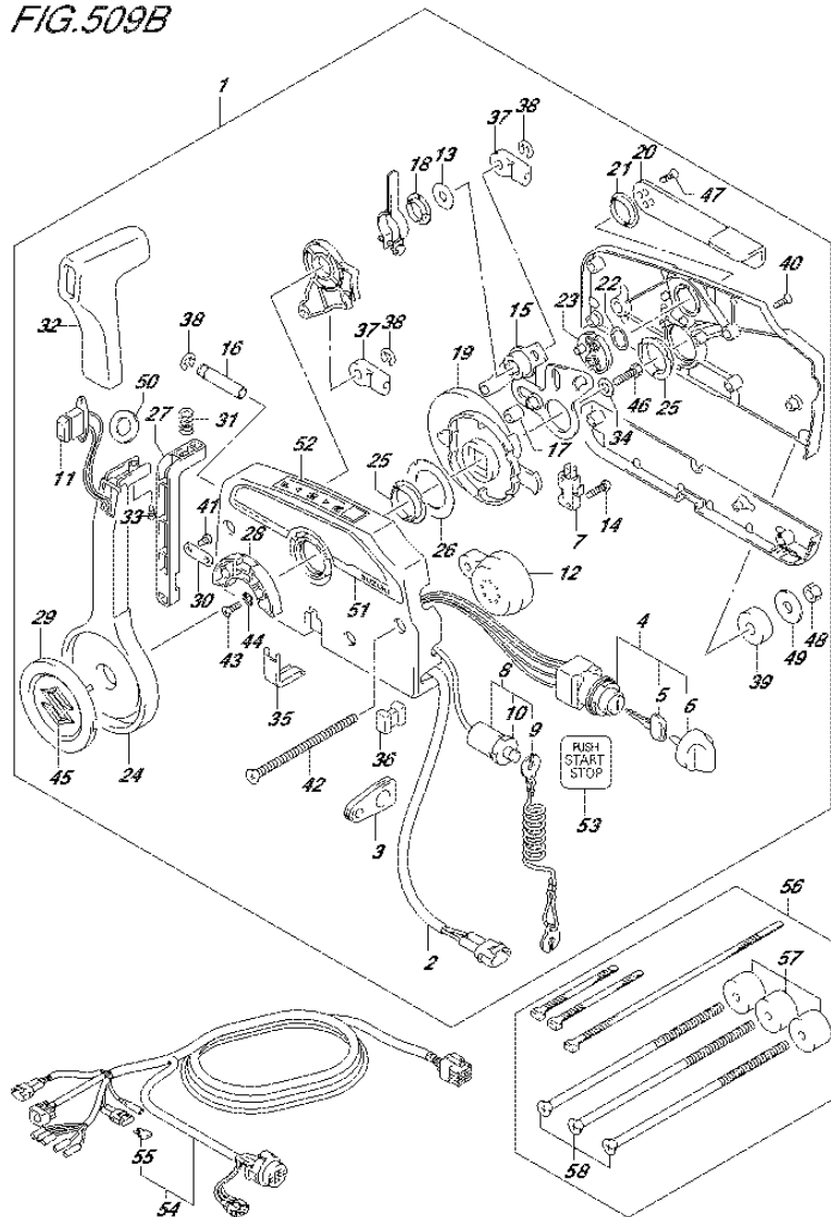
FIG.509B (3-C-10) OPT:REMOTE CONTROL (1) (DF115AT E11)
