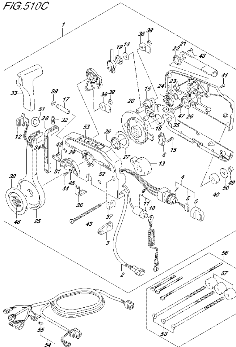
FIG.510C (3-D-14) OPT:REMOTE CONTROL (2) (DF115AT E40)
