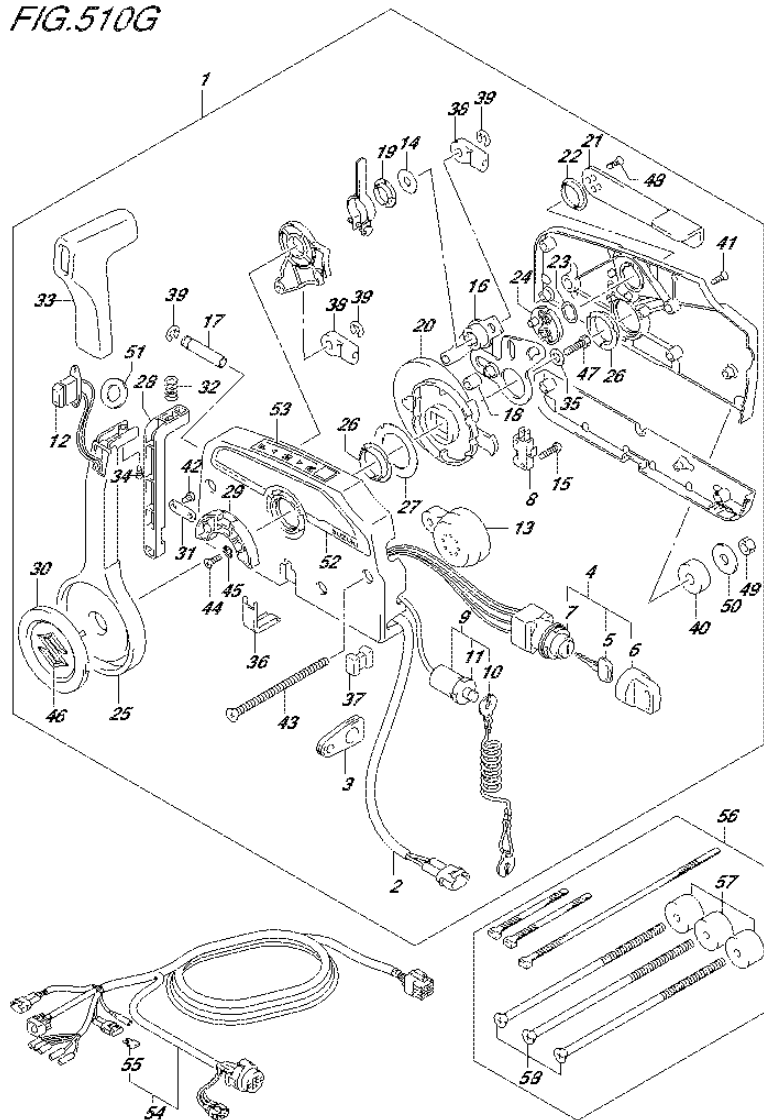
FIG.510G (3-E-11) OPT:REMOTE CONTROL (2) (DF140AT E40)
