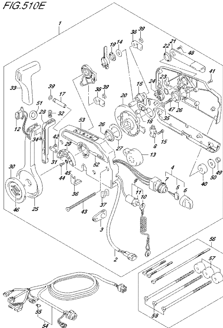
FIG.510E (3-E-4) OPT:REMOTE CONTROL (2) (DF115AZ E40)
