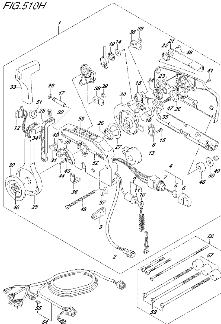
FIG.510H (3-E-13) OPT:REMOTE CONTROL (2) (DF140AZ E11)
