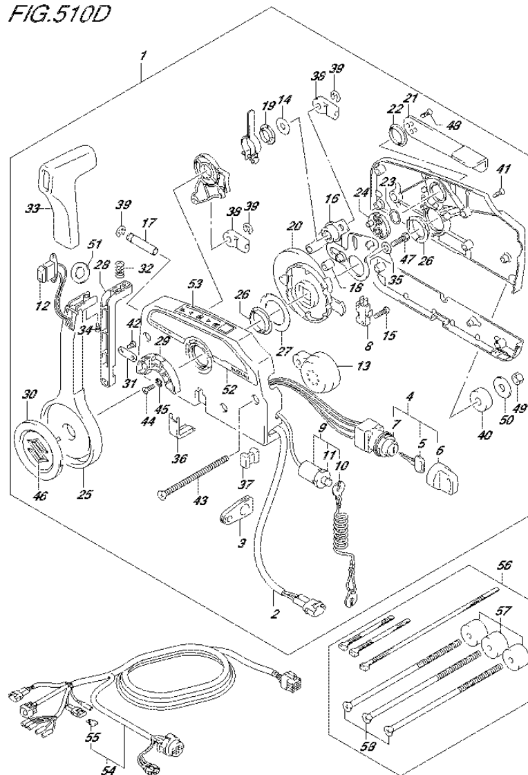
FIG.510D (3-D-15) OPT:REMOTE CONTROL (2) (DF115AZ E11)
