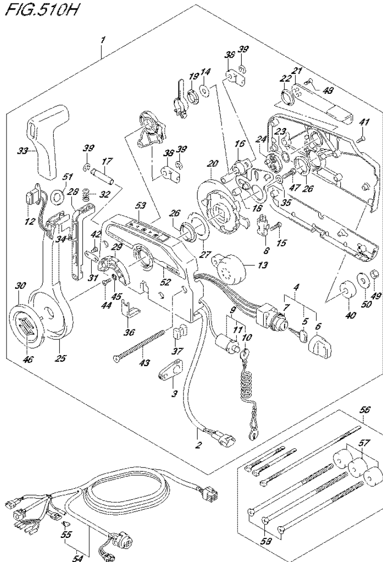
FIG.510H (3-E-14) OPT:REMOTE CONTROL (2) (DF140AZ E11)
