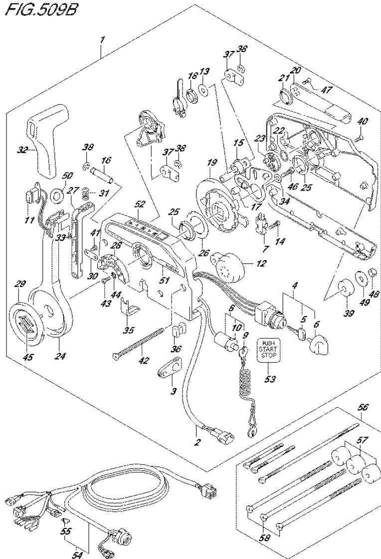
FIG.509B (3-C-8) OPT:REMOTE CONTROL (1) (DF115AT E11)
