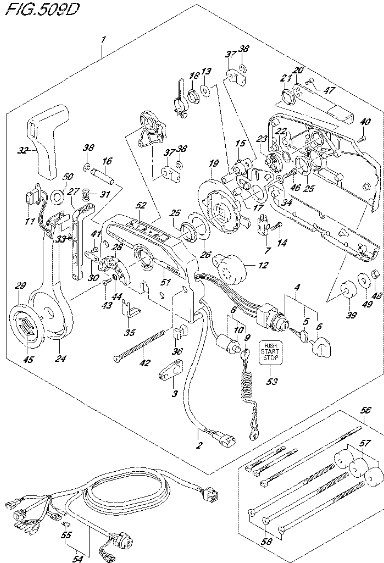
FIG.509D (3-D-2) OPT:REMOTE CONTROL (1) (DF140AT E11)
