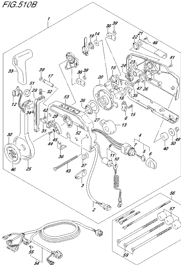
FIG.510B (3-D-9) OPT:REMOTE CONTROL (2) (DF115AT E11)
