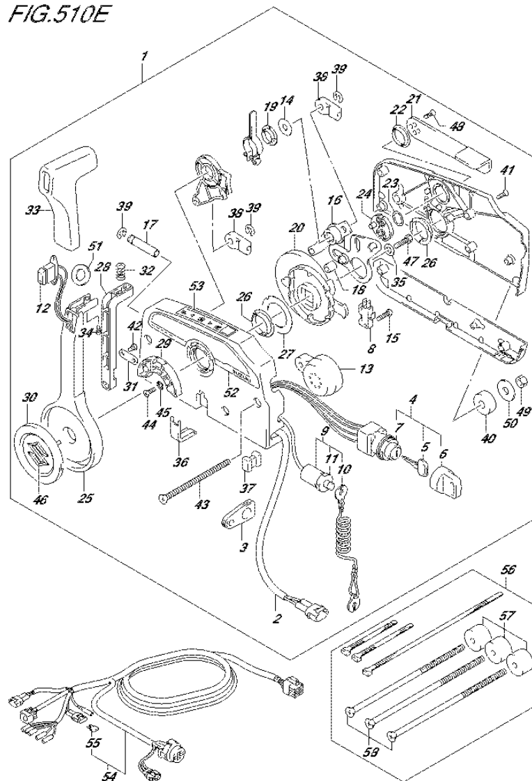
FIG.510E (3-E-5) OPT:REMOTE CONTROL (2) (DF115AZ E40)
