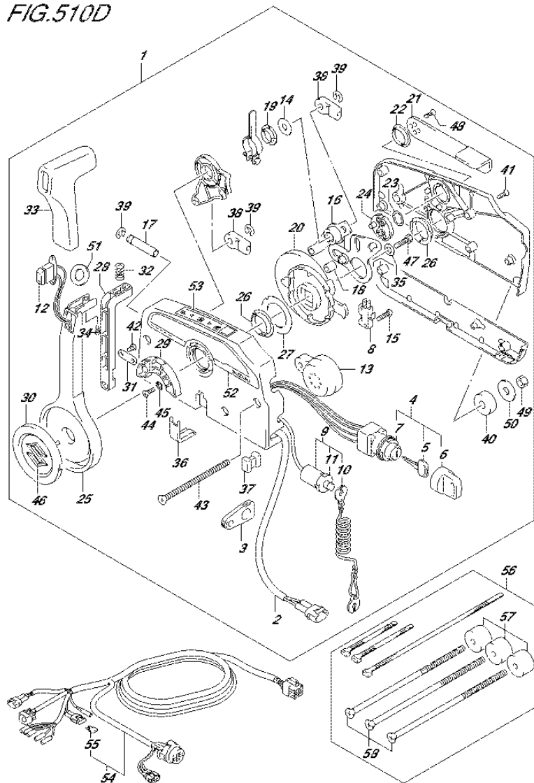
FIG.510D (3-E-3) OPT:REMOTE CONTROL (2) (DF115AZ E11)
