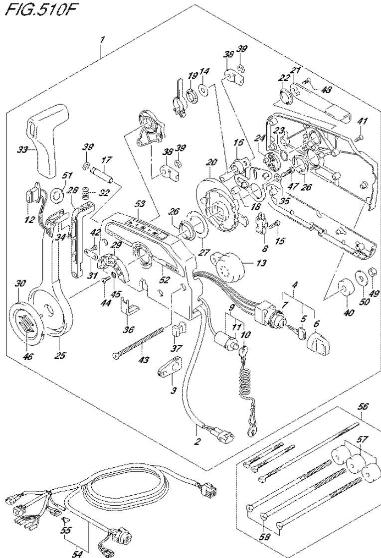
FIG.510F (3-E-8) OPT:REMOTE CONTROL (2) (DF140AT E11)
