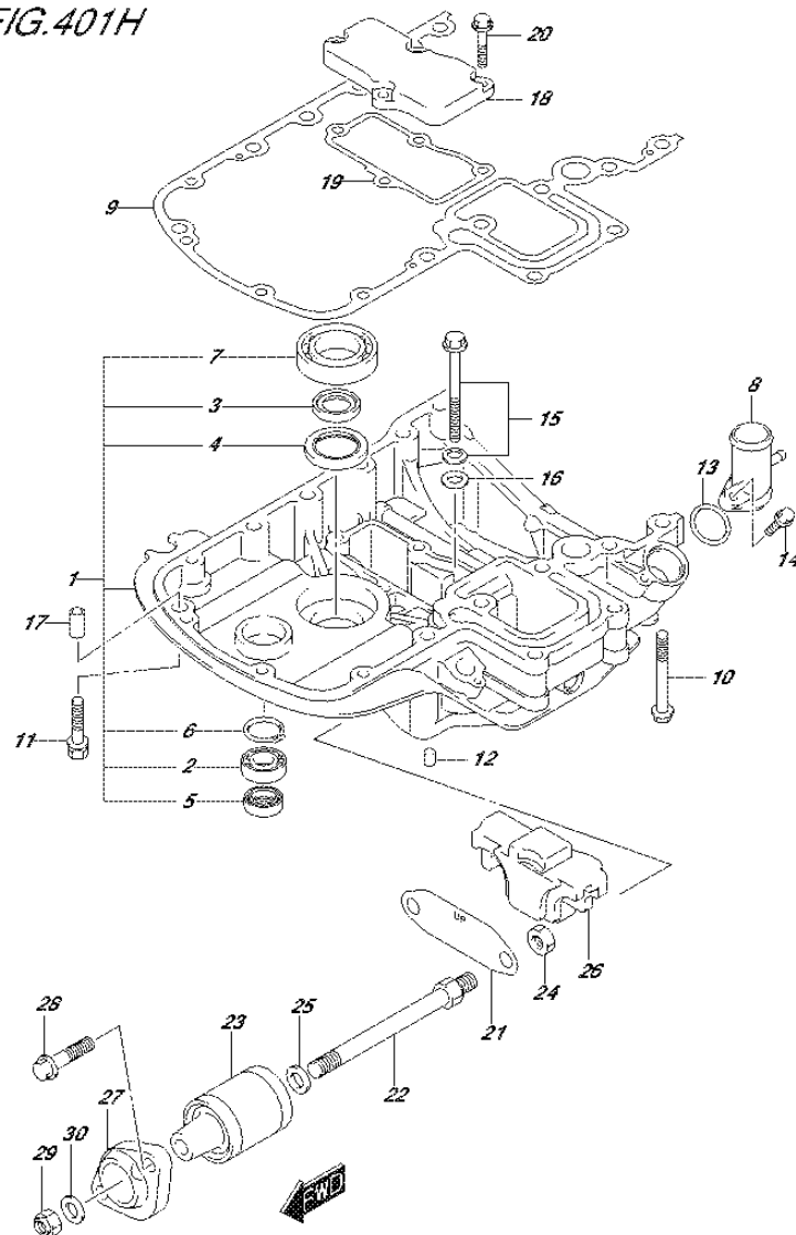
FIG.401H (2-F-13) ENGINE HOLDER (DF140AZ E11)
