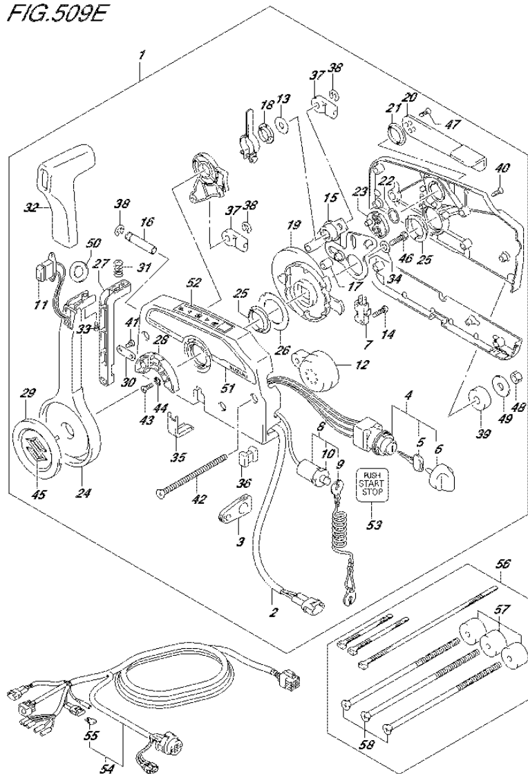
FIG.509E (3-D-4) OPT:REMOTE CONTROL (1) (DF140AZ E11)
