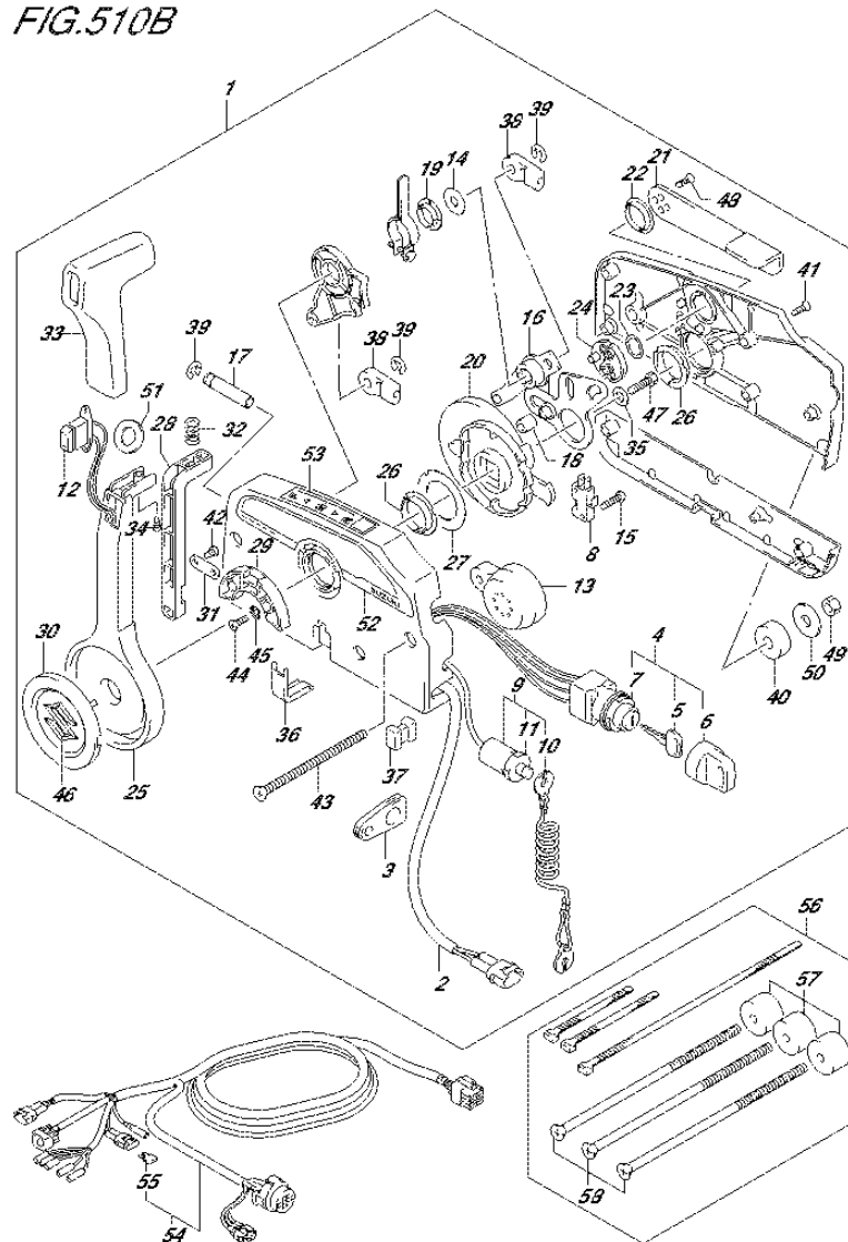
FIG.510B (3-D-11) OPT:REMOTE CONTROL (2) (DF115AT E11)
