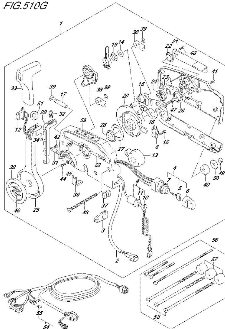
FIG.510G (3-E-12) OPT:REMOTE CONTROL (2) (DF140AT E40)
